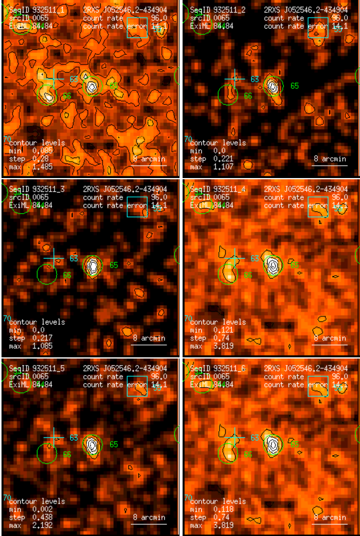
Figure 65: RASS 932511: detection 0065: band rate images, Gaussian filter: (1) PSPC channels 11 – 41, (2) 52 – 90, (3) 91 – 201, (4) 11 – 235, (5) 52 – 201, (6) 11 – 201. Broad band rates in counts/ks. Band rate contour levels in counts/ks/arcmin 2 .
