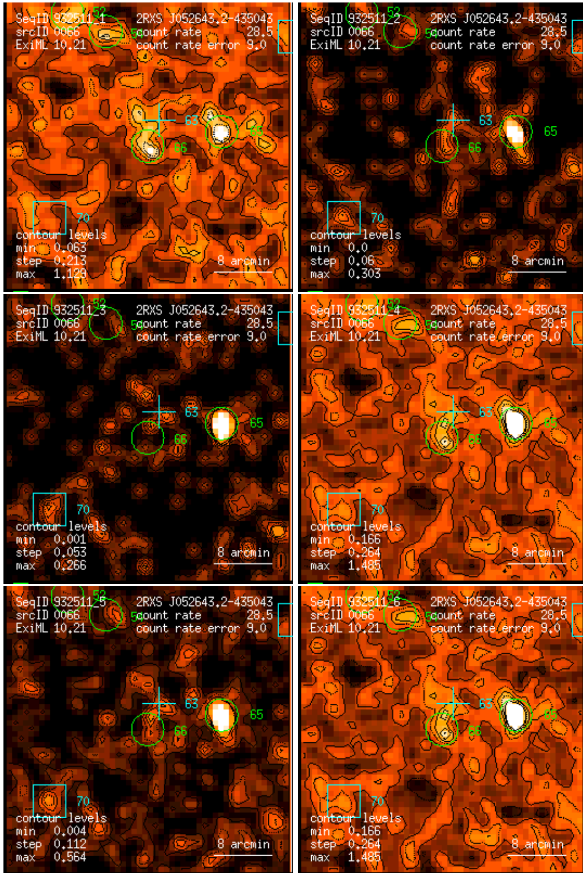
Figure 66: RASS 932511: detection 0066: band rate images, Gaussian filter: (1) PSPC channels 11 – 41, (2) 52 – 90, (3) 91 – 201, (4) 11 – 235, (5) 52 – 201, (6) 11 – 201. Broad band rates in counts/ks. Band rate contour levels in counts/ks/arcmin 2 .
