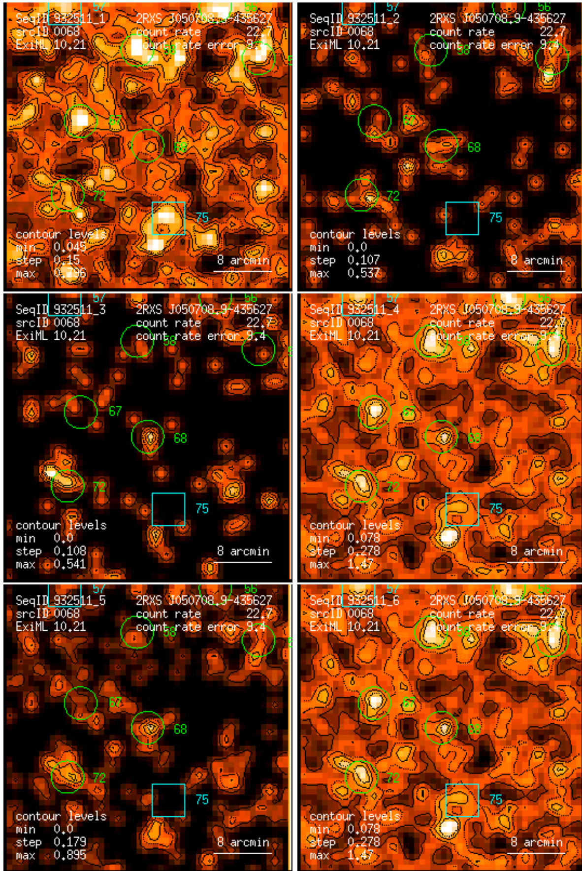
Figure 68: RASS 932511: detection 0068: band rate images, Gaussian filter: (1) PSPC channels 11 – 41, (2) 52 – 90, (3) 91 – 201, (4) 11 – 235, (5) 52 – 201, (6) 11 – 201. Broad band rates in counts/ks. Band rate contour levels in counts/ks/arcmin 2 .
