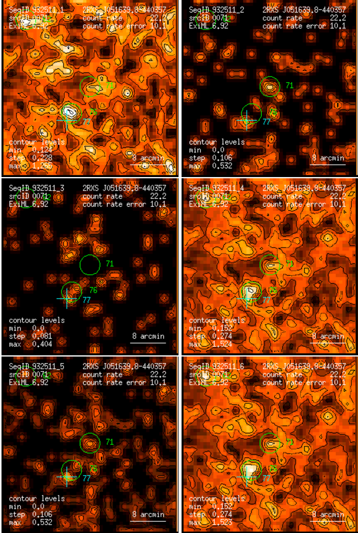
Figure 71: RASS 932511: detection 0071: band rate images, Gaussian filter: (1) PSPC channels 11 – 41, (2) 52 – 90, (3) 91 – 201, (4) 11 – 235, (5) 52 – 201, (6) 11 – 201. Broad band rates in counts/ks. Band rate contour levels in counts/ks/arcmin 2 .
