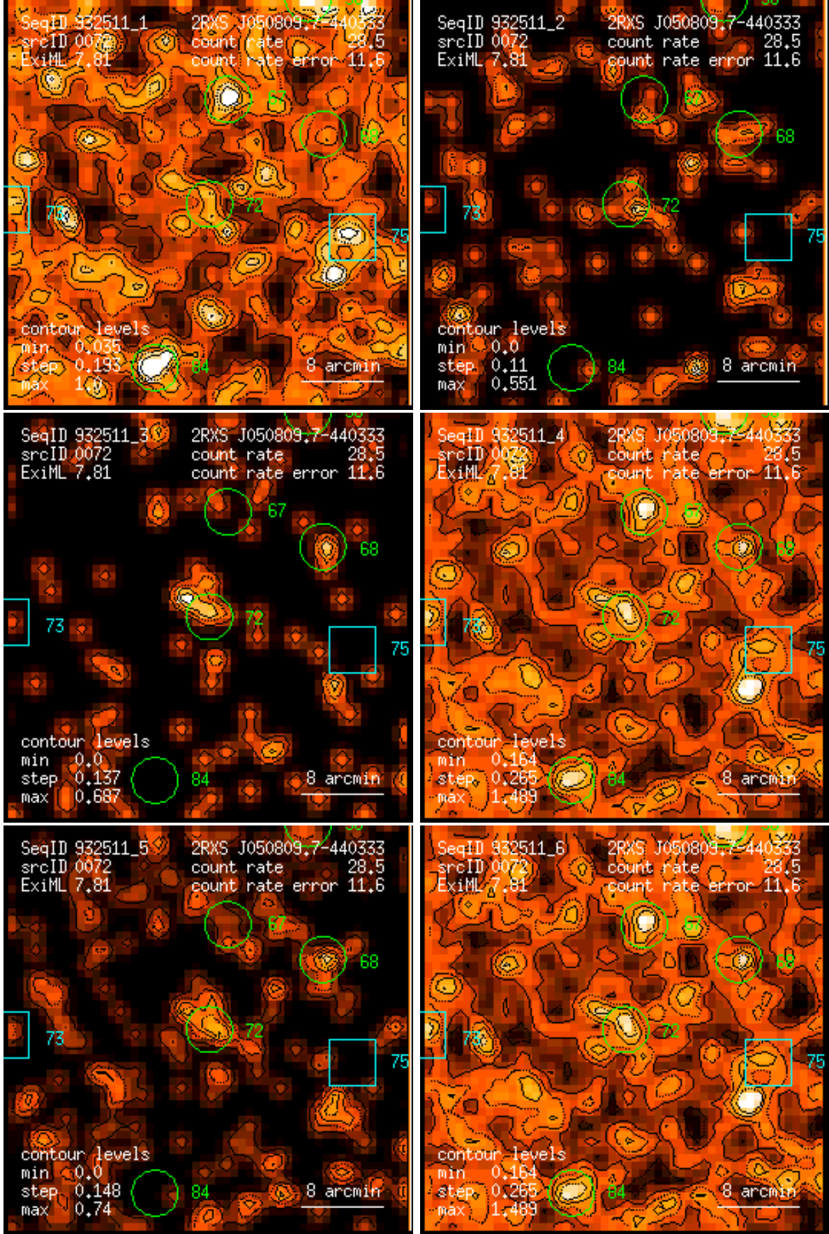
Figure 72: RASS 932511: detection 0072: band rate images, Gaussian filter: (1) PSPC channels 11 – 41, (2) 52 – 90, (3) 91 – 201, (4) 11 – 235, (5) 52 – 201, (6) 11 – 201. Broad band rates in counts/ks. Band rate contour levels in counts/ks/arcmin 2 .
