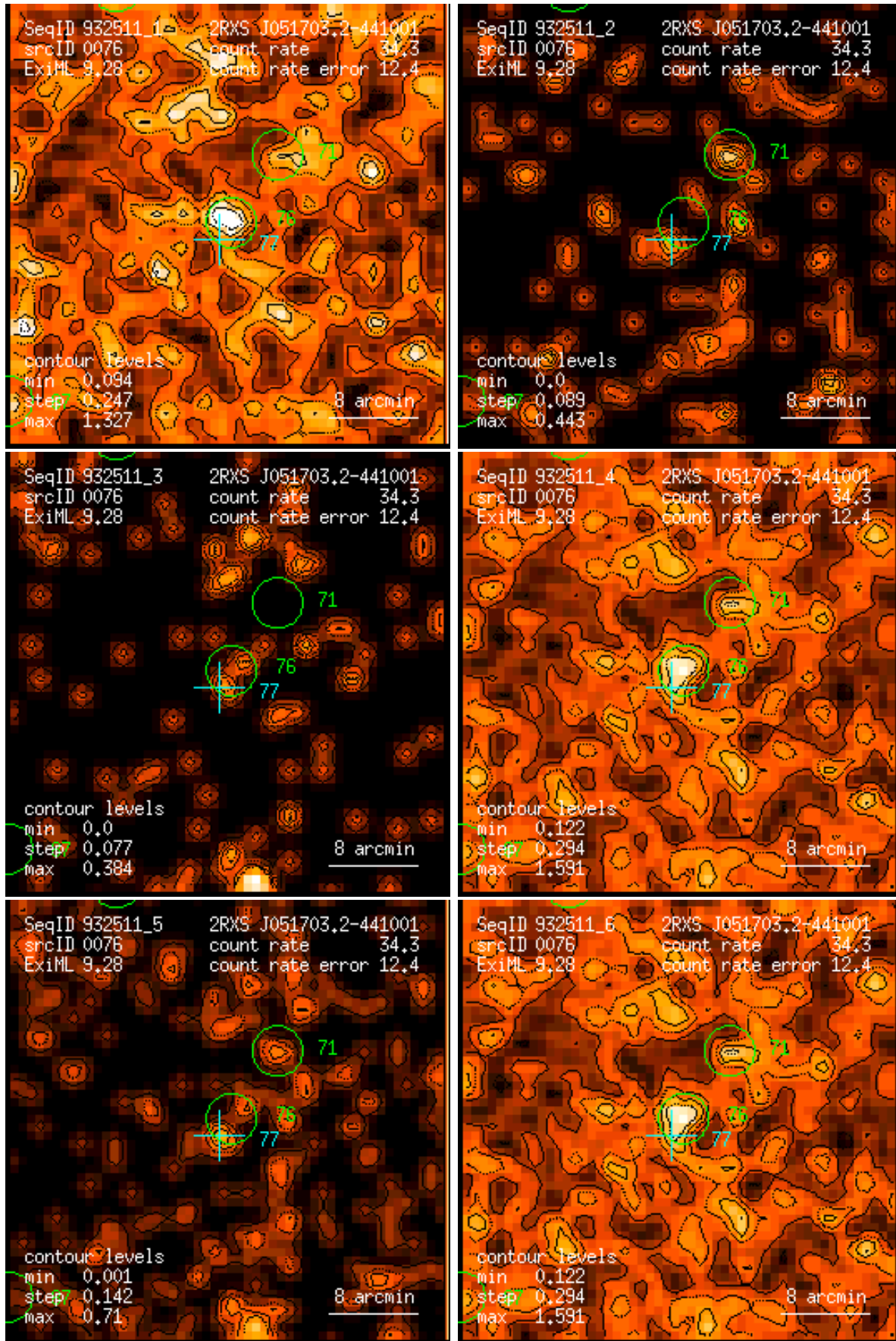
Figure 76: RASS 932511: detection 0076: band rate images, Gaussian filter: (1) PSPC channels 11 – 41, (2) 52 – 90, (3) 91 – 201, (4) 11 – 235, (5) 52 – 201, (6) 11 – 201. Broad band rates in counts/ks. Band rate contour levels in counts/ks/arcmin 2 .
