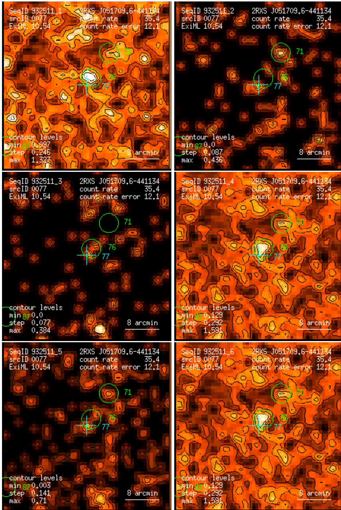
Figure 77: RASS 932511: detection 0077: band rate images, Gaussian filter: (1) PSPC channels 11 – 41, (2) 52 – 90, (3) 91 – 201, (4) 11 – 235, (5) 52 – 201, (6) 11 – 201. Broad band rates in counts/ks. Band rate contour levels in counts/ks/arcmin 2 .
