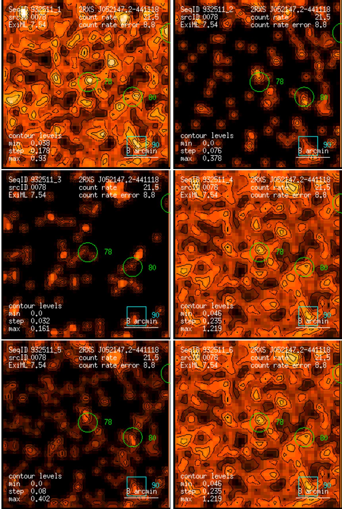
Figure 78: RASS 932511: detection 0078: band rate images, Gaussian filter: (1) PSPC channels 11 – 41, (2) 52 – 90, (3) 91 – 201, (4) 11 – 235, (5) 52 – 201, (6) 11 – 201. Broad band rates in counts/ks. Band rate contour levels in counts/ks/arcmin 2 .
