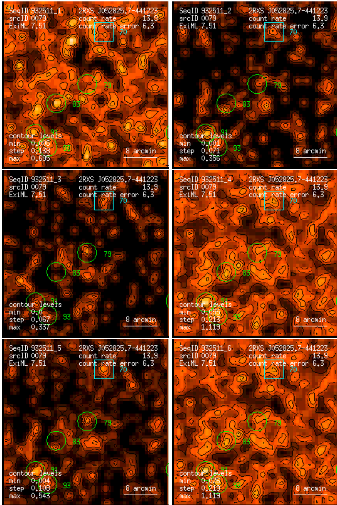
Figure 79: RASS 932511: detection 0079: band rate images, Gaussian filter: (1) PSPC channels 11 – 41, (2) 52 – 90, (3) 91 – 201, (4) 11 – 235, (5) 52 – 201, (6) 11 – 201. Broad band rates in counts/ks. Band rate contour levels in counts/ks/arcmin 2 .
