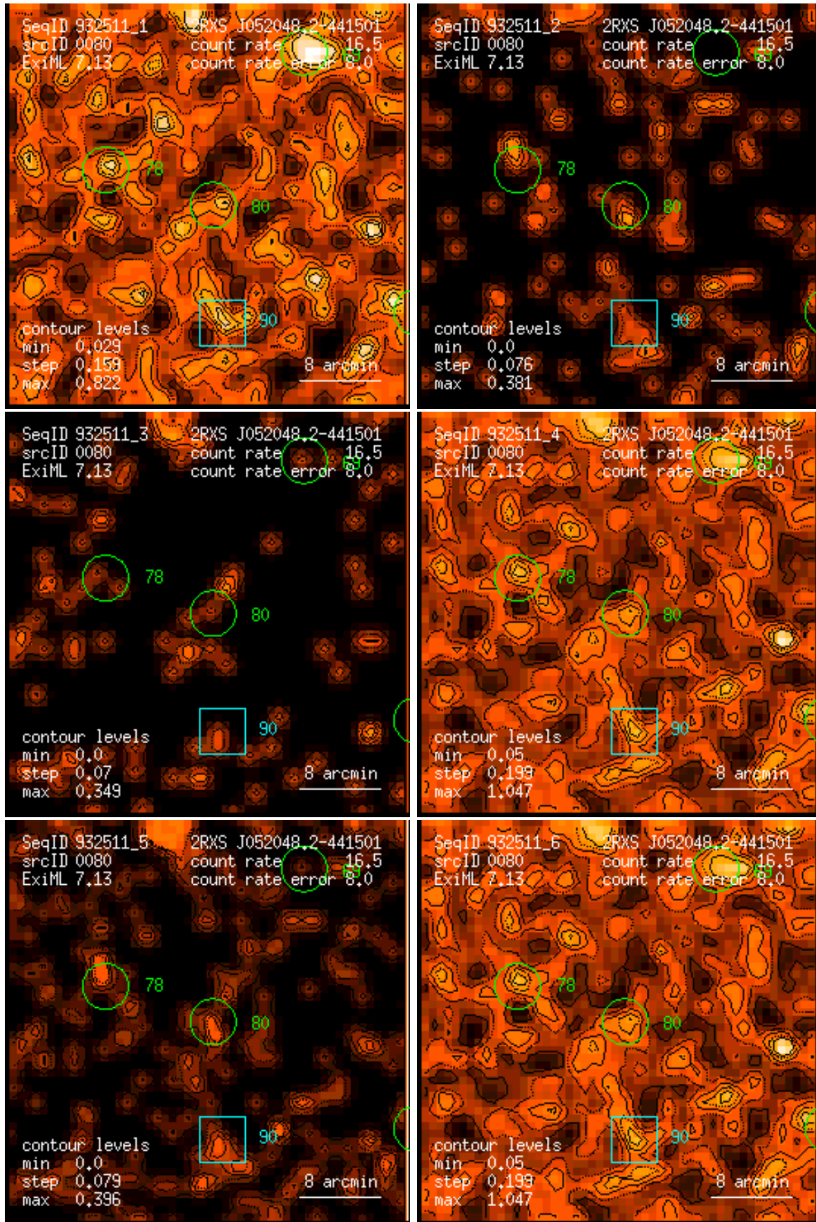
Figure 80: RASS 932511: detection 0080: band rate images, Gaussian filter: (1) PSPC channels 11 – 41, (2) 52 – 90, (3) 91 – 201, (4) 11 – 235, (5) 52 – 201, (6) 11 – 201. Broad band rates in counts/ks. Band rate contour levels in counts/ks/arcmin 2 .
