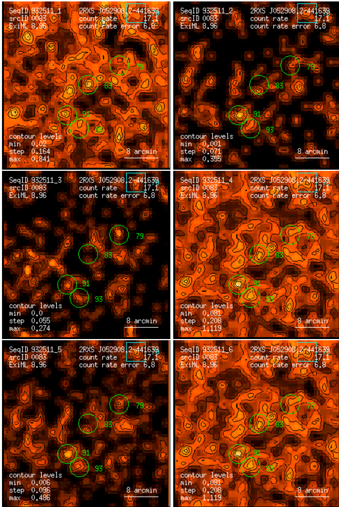
Figure 83: RASS 932511: detection 0083: band rate images, Gaussian filter: (1) PSPC channels 11 – 41, (2) 52 – 90, (3) 91 – 201, (4) 11 – 235, (5) 52 – 201, (6) 11 – 201. Broad band rates in counts/ks. Band rate contour levels in counts/ks/arcmin 2 .
