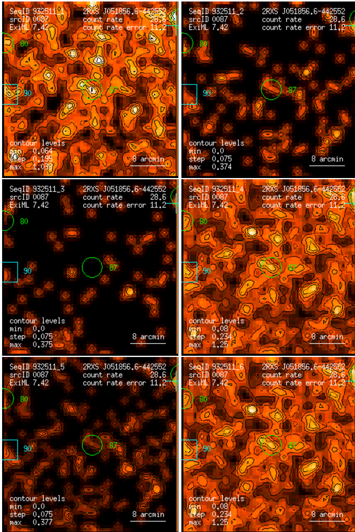
Figure 87: RASS 932511: detection 0087: band rate images, Gaussian filter: (1) PSPC channels 11 – 41, (2) 52 – 90, (3) 91 – 201, (4) 11 – 235, (5) 52 – 201, (6) 11 – 201. Broad band rates in counts/ks. Band rate contour levels in counts/ks/arcmin 2 .
