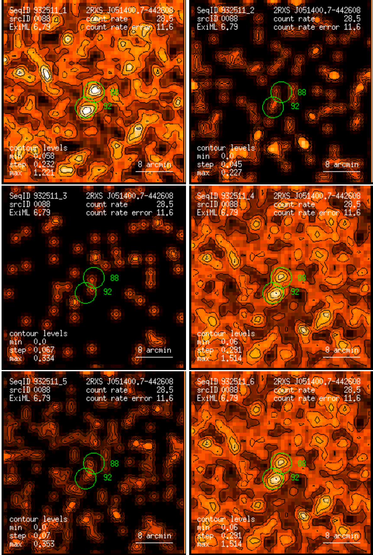
Figure 88: RASS 932511: detection 0088: band rate images, Gaussian filter: (1) PSPC channels 11 – 41, (2) 52 – 90, (3) 91 – 201, (4) 11 – 235, (5) 52 – 201, (6) 11 – 201. Broad band rates in counts/ks. Band rate contour levels in counts/ks/arcmin 2 .
