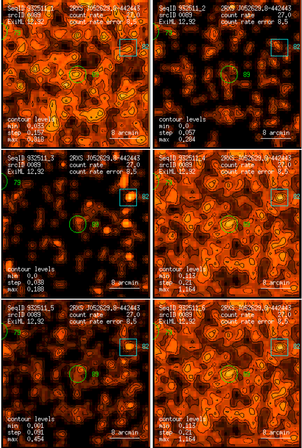
Figure 89: RASS 932511: detection 0089: band rate images, Gaussian filter: (1) PSPC channels 11 – 41, (2) 52 – 90, (3) 91 – 201, (4) 11 – 235, (5) 52 – 201, (6) 11 – 201. Broad band rates in counts/ks. Band rate contour levels in counts/ks/arcmin 2 .
