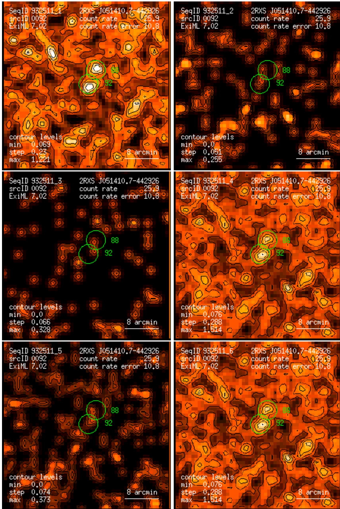
Figure 92: RASS 932511: detection 0092: band rate images, Gaussian filter: (1) PSPC channels 11 – 41, (2) 52 – 90, (3) 91 – 201, (4) 11 – 235, (5) 52 – 201, (6) 11 – 201. Broad band rates in counts/ks. Band rate contour levels in counts/ks/arcmin 2 .
