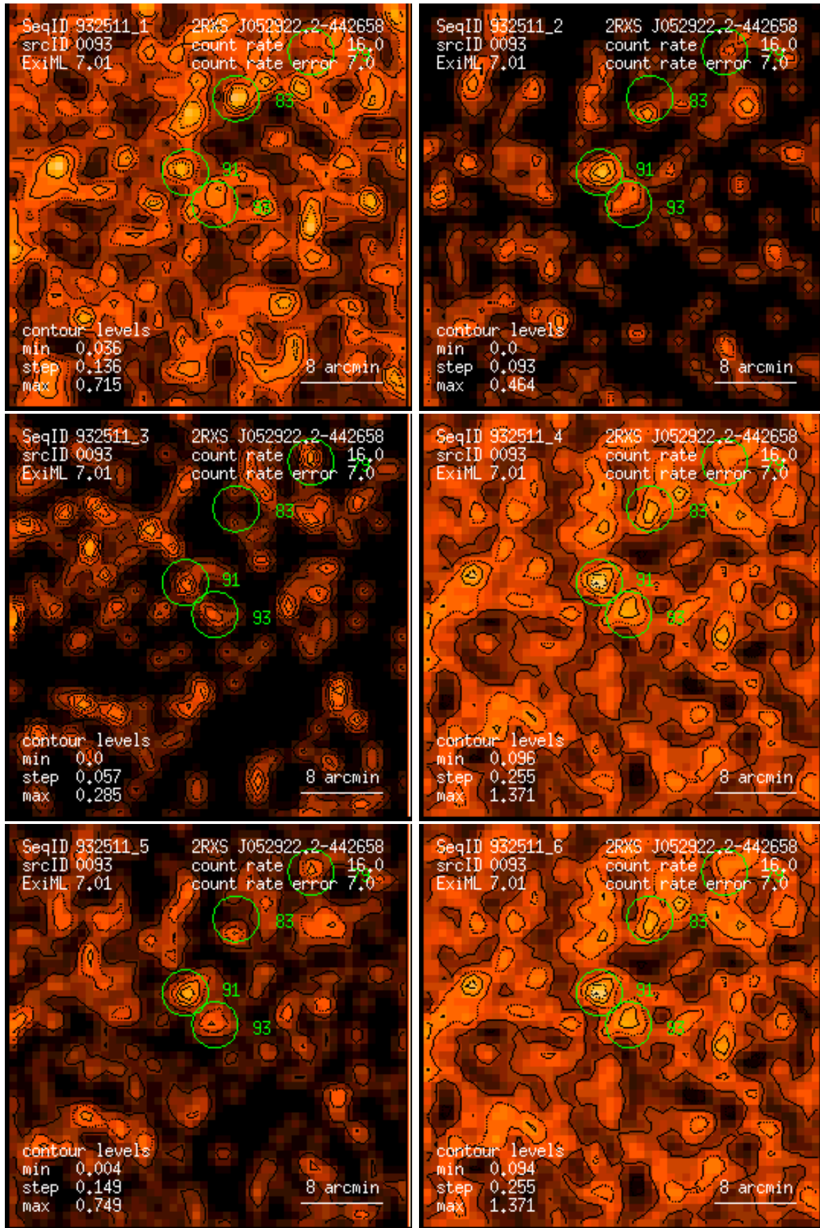
Figure 93: RASS 932511: detection 0093: band rate images, Gaussian filter: (1) PSPC channels 11 – 41, (2) 52 – 90, (3) 91 – 201, (4) 11 – 235, (5) 52 – 201, (6) 11 – 201. Broad band rates in counts/ks. Band rate contour levels in counts/ks/arcmin 2 .
