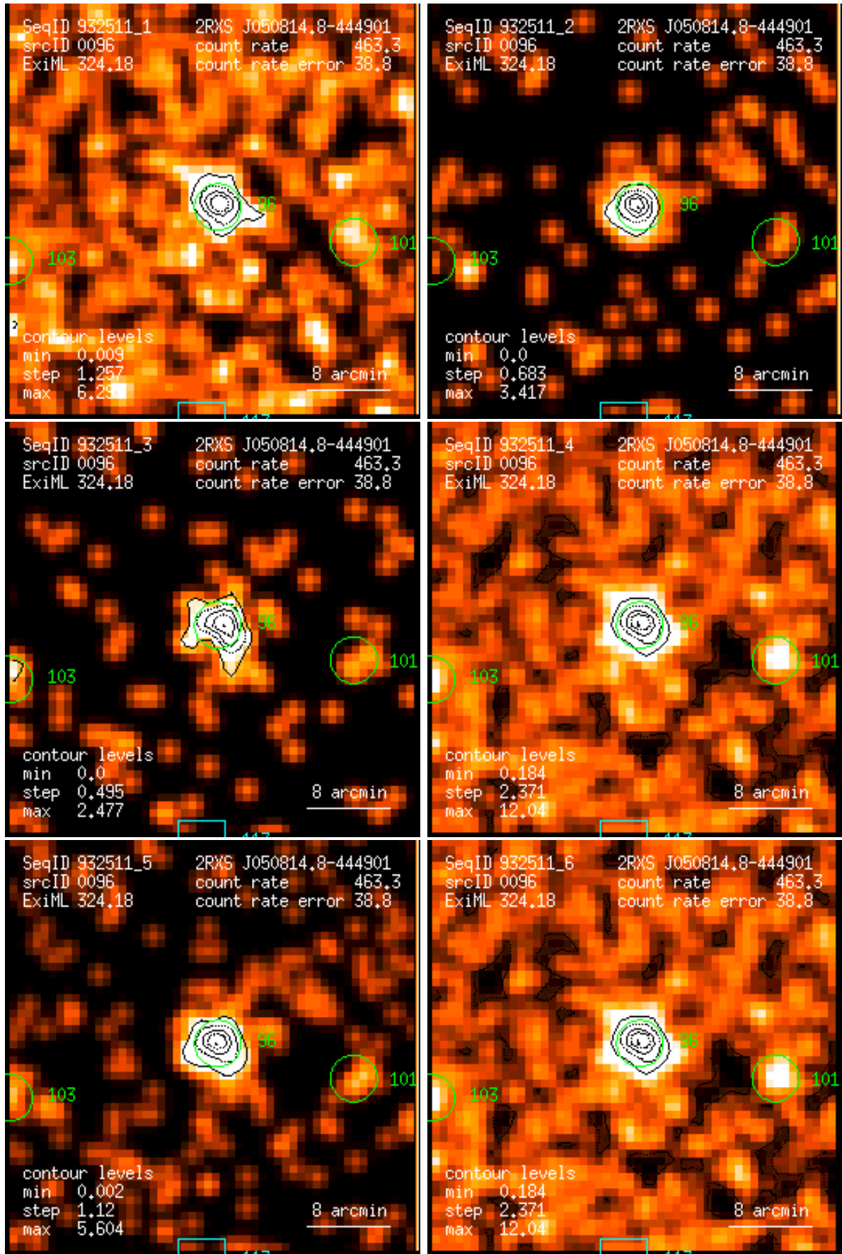
Figure 96: RASS 932511: detection 0096: band rate images, Gaussian filter: (1) PSPC channels 11 – 41, (2) 52 – 90, (3) 91 – 201, (4) 11 – 235, (5) 52 – 201, (6) 11 – 201. Broad band rates in counts/ks. Band rate contour levels in counts/ks/arcmin 2 .
