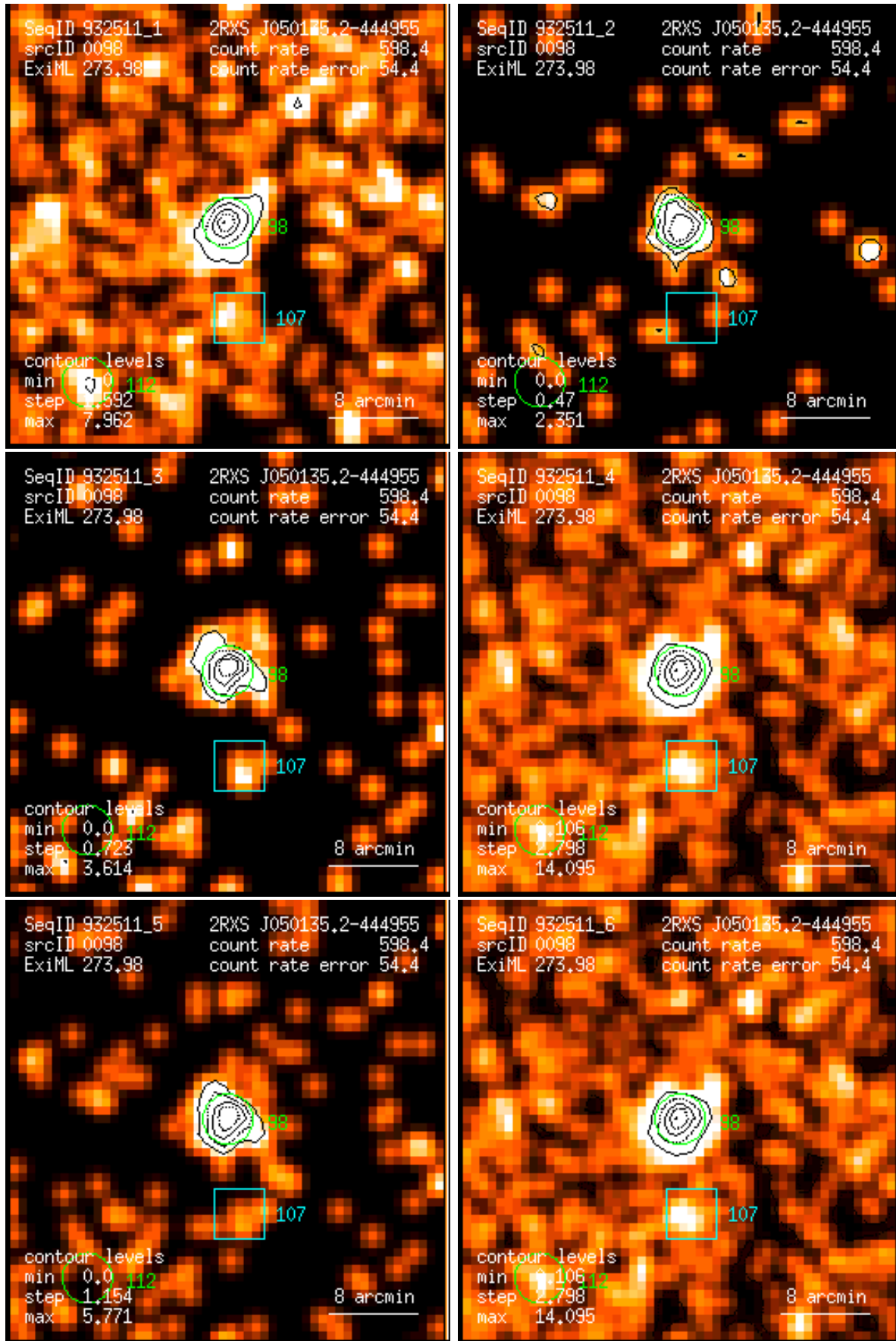
Figure 98: RASS 932511: detection 0098: band rate images, Gaussian filter: (1) PSPC channels 11 – 41, (2) 52 – 90, (3) 91 – 201, (4) 11 – 235, (5) 52 – 201, (6) 11 – 201. Broad band rates in counts/ks. Band rate contour levels in counts/ks/arcmin 2 .
