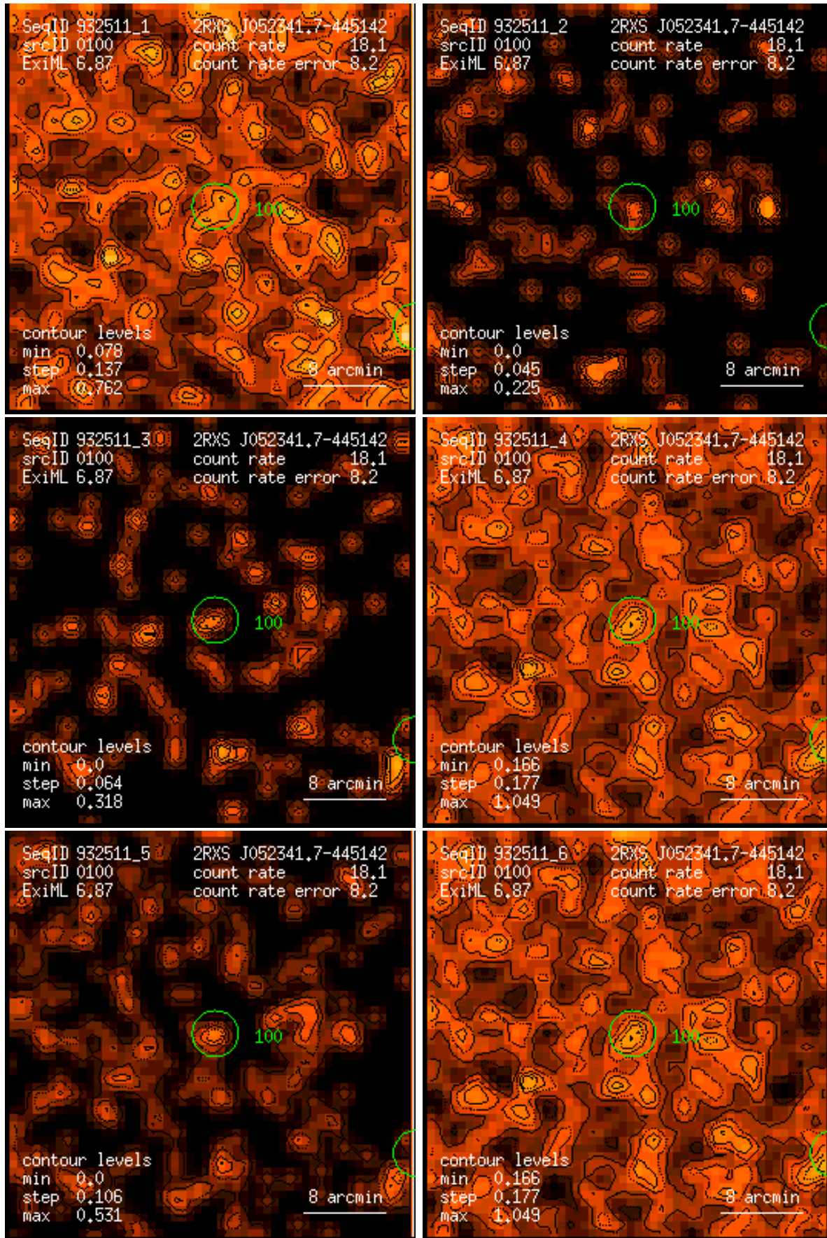
Figure 100: RASS 932511: detection 0100: band rate images, Gaussian filter: (1) PSPC channels 11 – 41, (2) 52 – 90, (3) 91 – 201, (4) 11 – 235, (5) 52 – 201, (6) 11 – 201. Broad band rates in counts/ks. Band rate contour levels in counts/ks/arcmin 2 .
