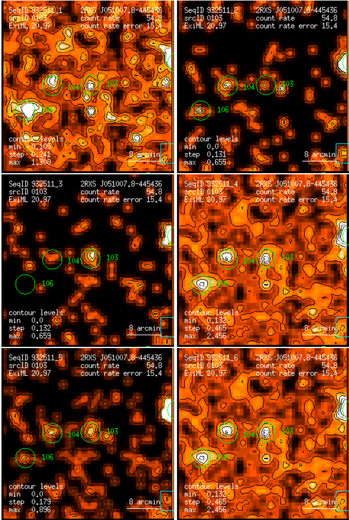
Figure 103: RASS 932511: detection 0103: band rate images, Gaussian filter: (1) PSPC channels 11 – 41, (2) 52 – 90, (3) 91 – 201, (4) 11 – 235, (5) 52 – 201, (6) 11 – 201. Broad band rates in counts/ks. Band rate contour levels in counts/ks/arcmin 2 .
