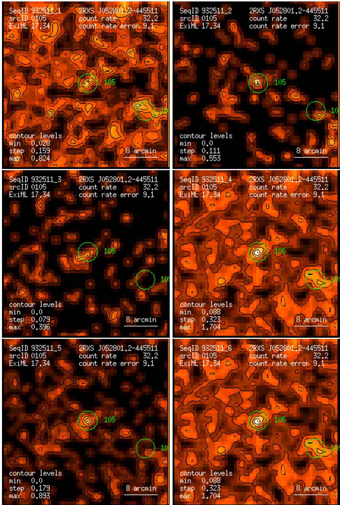
Figure 105: RASS 932511: detection 0105: band rate images, Gaussian filter: (1) PSPC channels 11 – 41, (2) 52 – 90, (3) 91 – 201, (4) 11 – 235, (5) 52 – 201, (6) 11 – 201. Broad band rates in counts/ks. Band rate contour levels in counts/ks/arcmin 2 .
