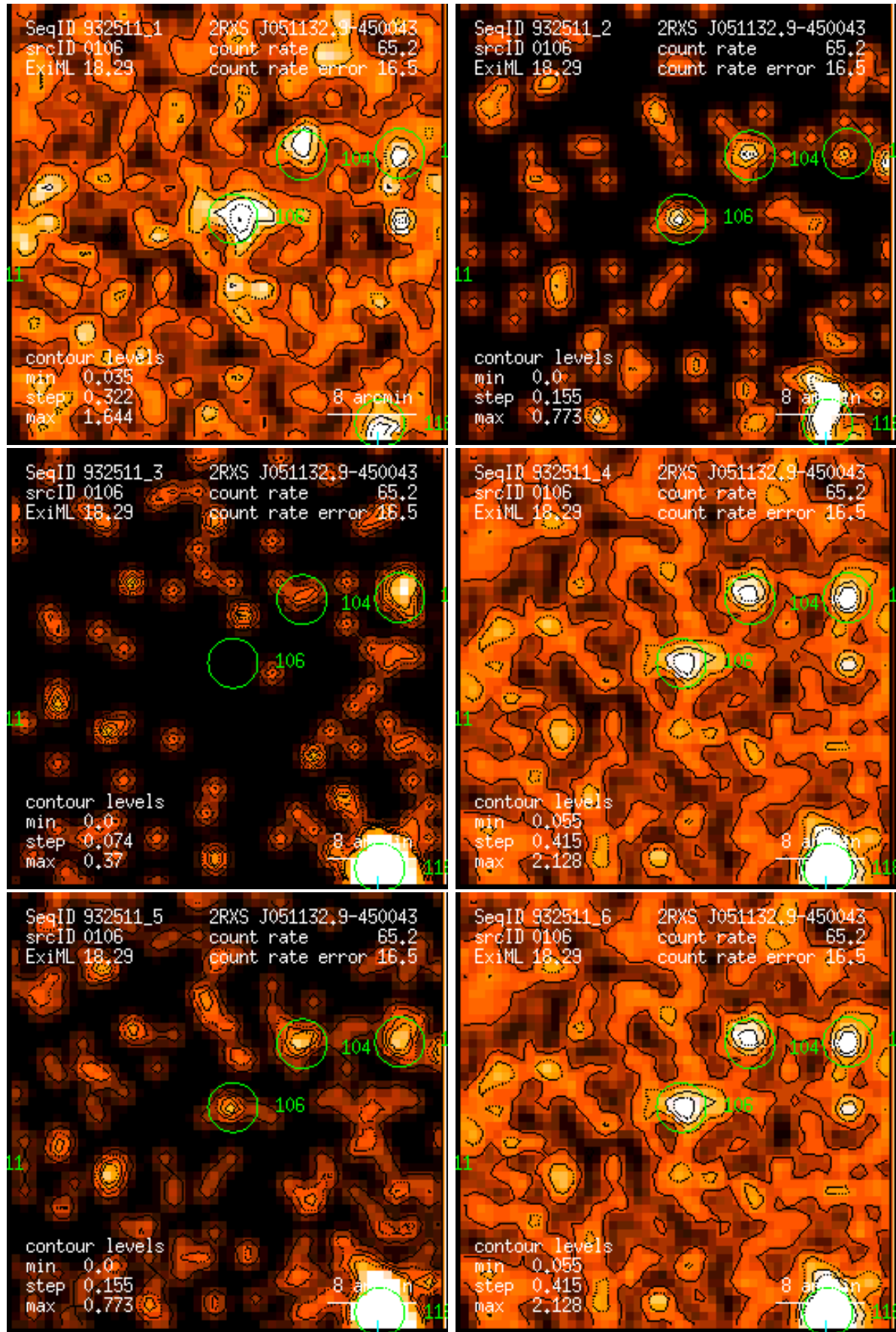
Figure 106: RASS 932511: detection 0106: band rate images, Gaussian filter: (1) PSPC channels 11 – 41, (2) 52 – 90, (3) 91 – 201, (4) 11 – 235, (5) 52 – 201, (6) 11 – 201. Broad band rates in counts/ks. Band rate contour levels in counts/ks/arcmin 2 .
