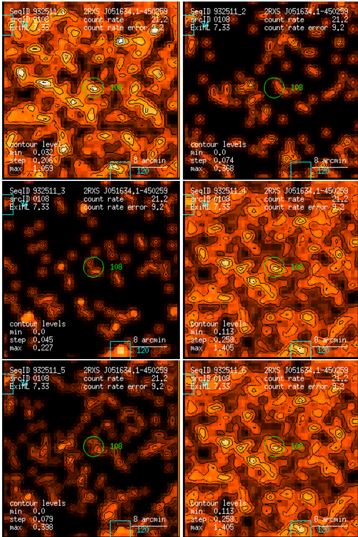
Figure 108: RASS 932511: detection 0108: band rate images, Gaussian filter: (1) PSPC channels 11 – 41, (2) 52 – 90, (3) 91 – 201, (4) 11 – 235, (5) 52 – 201, (6) 11 – 201. Broad band rates in counts/ks. Band rate contour levels in counts/ks/arcmin 2 .
