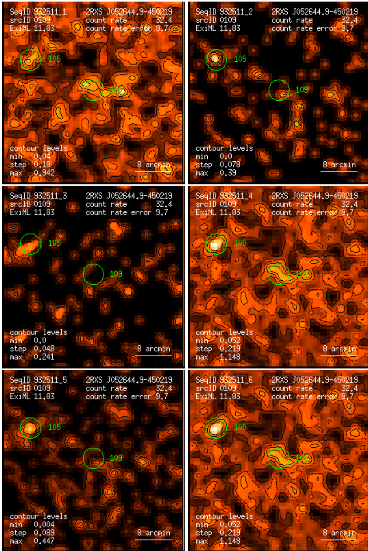
Figure 109: RASS 932511: detection 0109: band rate images, Gaussian filter: (1) PSPC channels 11 – 41, (2) 52 – 90, (3) 91 – 201, (4) 11 – 235, (5) 52 – 201, (6) 11 – 201. Broad band rates in counts/ks. Band rate contour levels in counts/ks/arcmin 2 .
