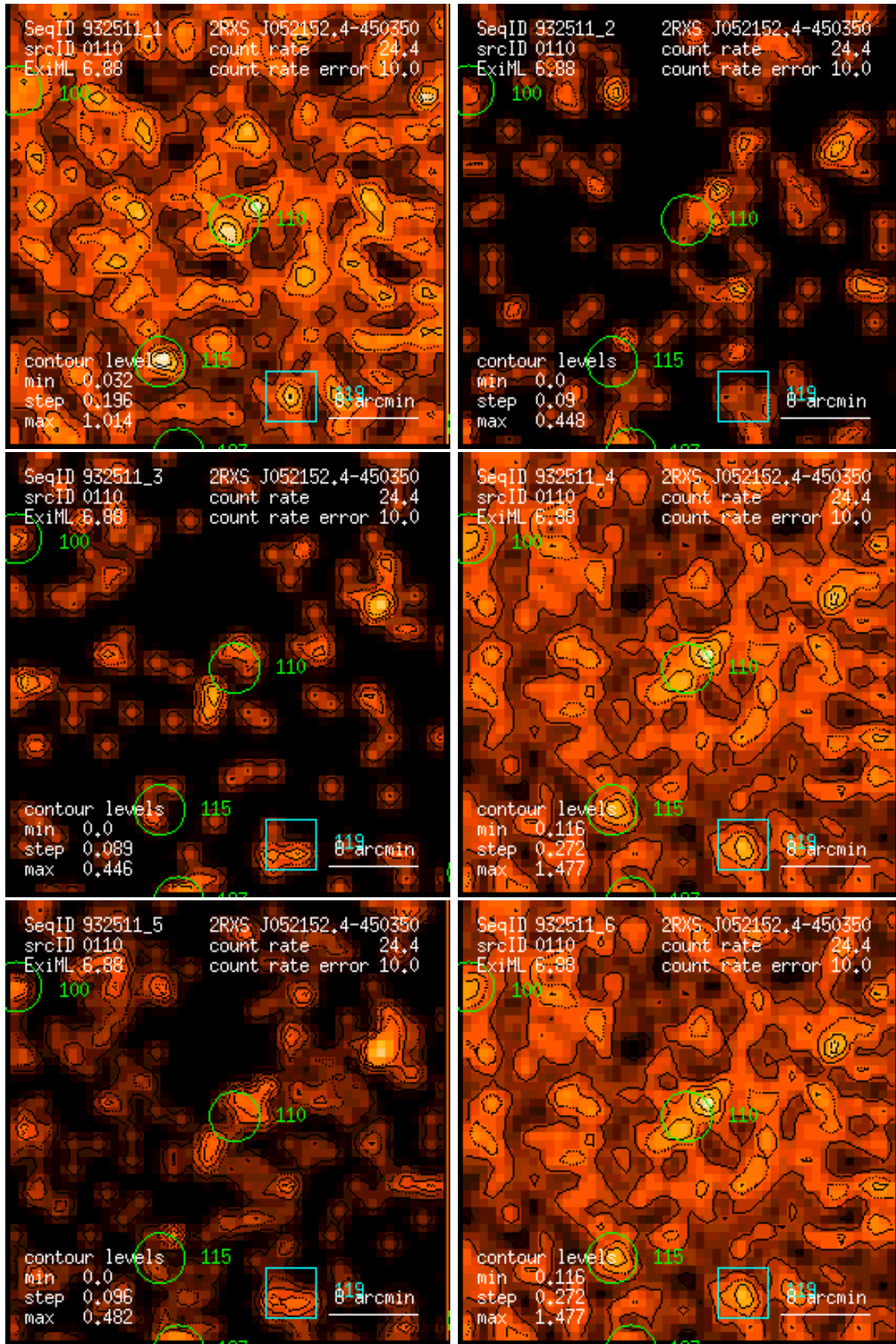
Figure 110: RASS 932511: detection 0110: band rate images, Gaussian filter: (1) PSPC channels 11 – 41, (2) 52 – 90, (3) 91 – 201, (4) 11 – 235, (5) 52 – 201, (6) 11 – 201. Broad band rates in counts/ks. Band rate contour levels in counts/ks/arcmin 2 .
