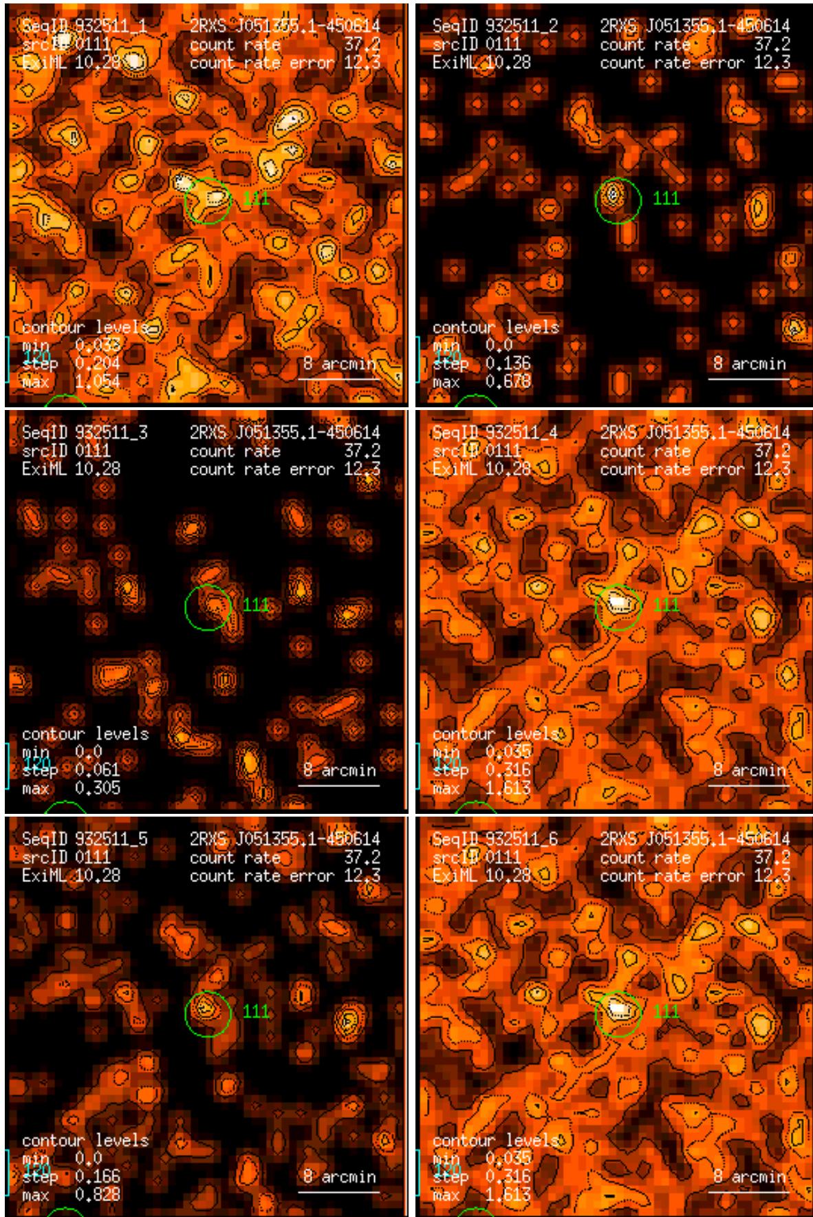
Figure 111: RASS 932511: detection 0111: band rate images, Gaussian filter: (1) PSPC channels 11 – 41, (2) 52 – 90, (3) 91 – 201, (4) 11 – 235, (5) 52 – 201, (6) 11 – 201. Broad band rates in counts/ks. Band rate contour levels in counts/ks/arcmin 2 .
