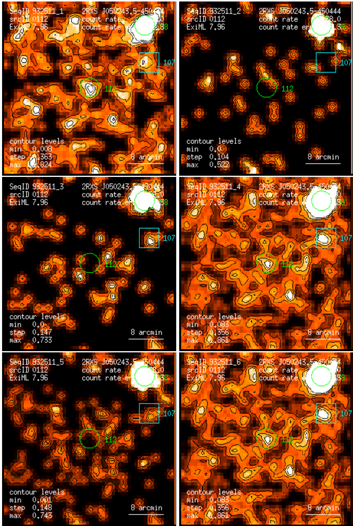
Figure 112: RASS 932511: detection 0112: band rate images, Gaussian filter: (1) PSPC channels 11 – 41, (2) 52 – 90, (3) 91 – 201, (4) 11 – 235, (5) 52 – 201, (6) 11 – 201. Broad band rates in counts/ks. Band rate contour levels in counts/ks/arcmin 2 .
