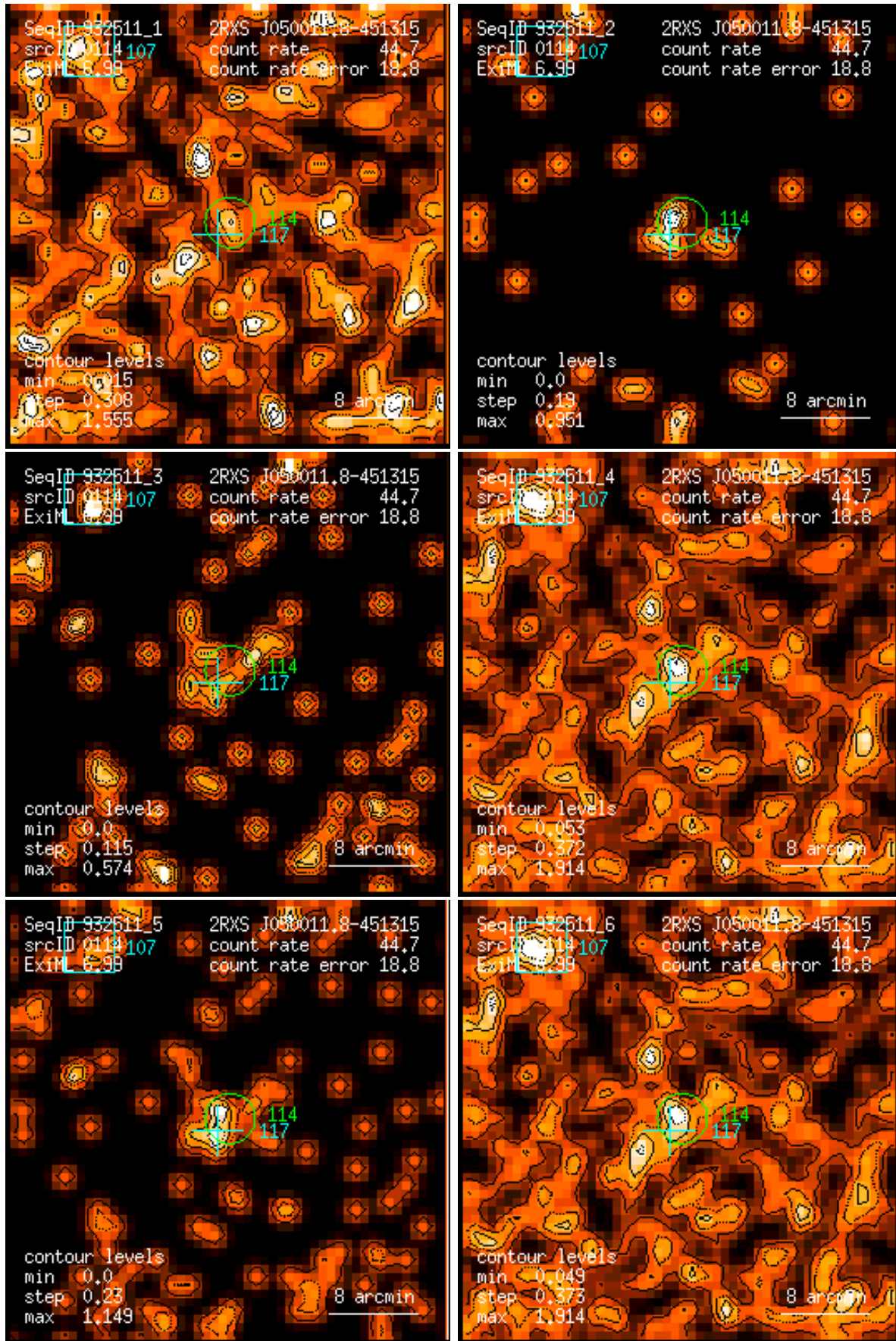
Figure 114: RASS 932511: detection 0114: band rate images, Gaussian filter: (1) PSPC channels 11 – 41, (2) 52 – 90, (3) 91 – 201, (4) 11 – 235, (5) 52 – 201, (6) 11 – 201. Broad band rates in counts/ks. Band rate contour levels in counts/ks/arcmin 2 .
