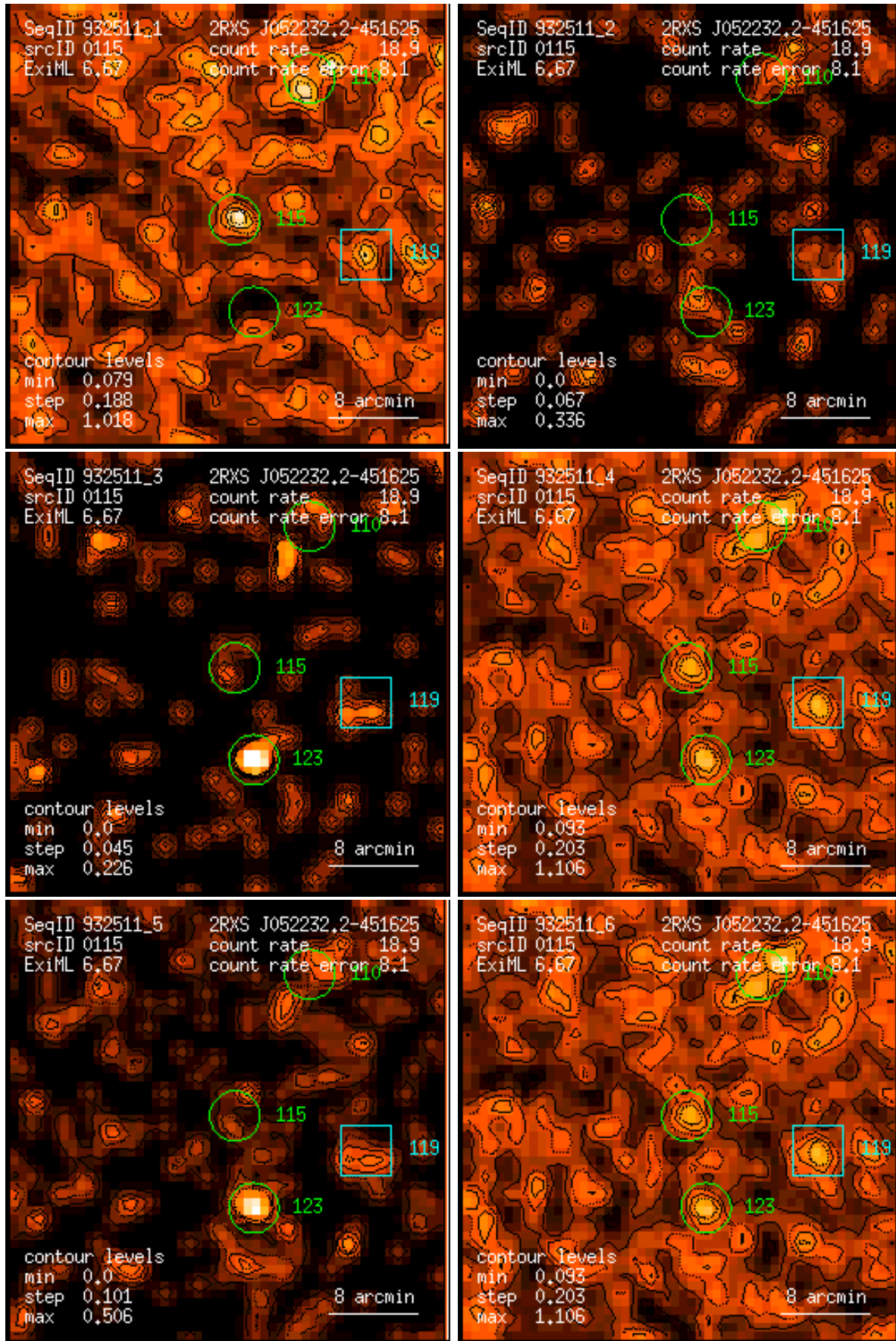
Figure 115: RASS 932511: detection 0115: band rate images, Gaussian filter: (1) PSPC channels 11 – 41, (2) 52 – 90, (3) 91 – 201, (4) 11 – 235, (5) 52 – 201, (6) 11 – 201. Broad band rates in counts/ks. Band rate contour levels in counts/ks/arcmin 2 .
