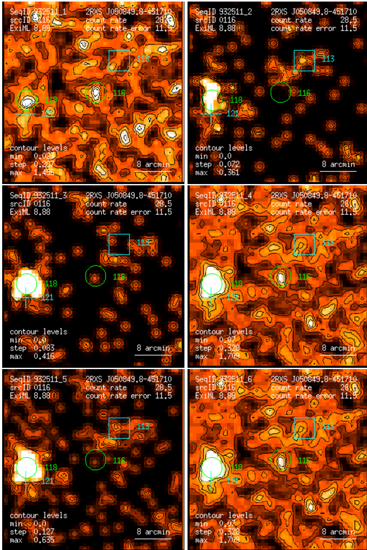
Figure 116: RASS 932511: detection 0116: band rate images, Gaussian filter: (1) PSPC channels 11 – 41, (2) 52 – 90, (3) 91 – 201, (4) 11 – 235, (5) 52 – 201, (6) 11 – 201. Broad band rates in counts/ks. Band rate contour levels in counts/ks/arcmin 2 .
