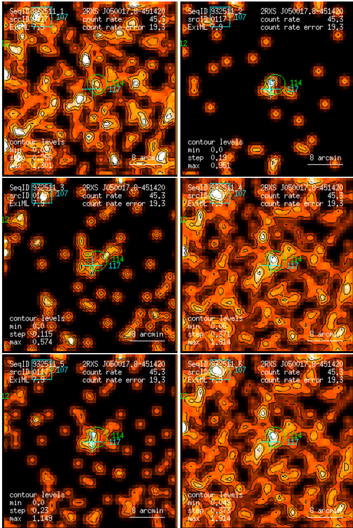
Figure 117: RASS 932511: detection 0117: band rate images, Gaussian filter: (1) PSPC channels 11 – 41, (2) 52 – 90, (3) 91 – 201, (4) 11 – 235, (5) 52 – 201, (6) 11 – 201. Broad band rates in counts/ks. Band rate contour levels in counts/ks/arcmin 2 .
