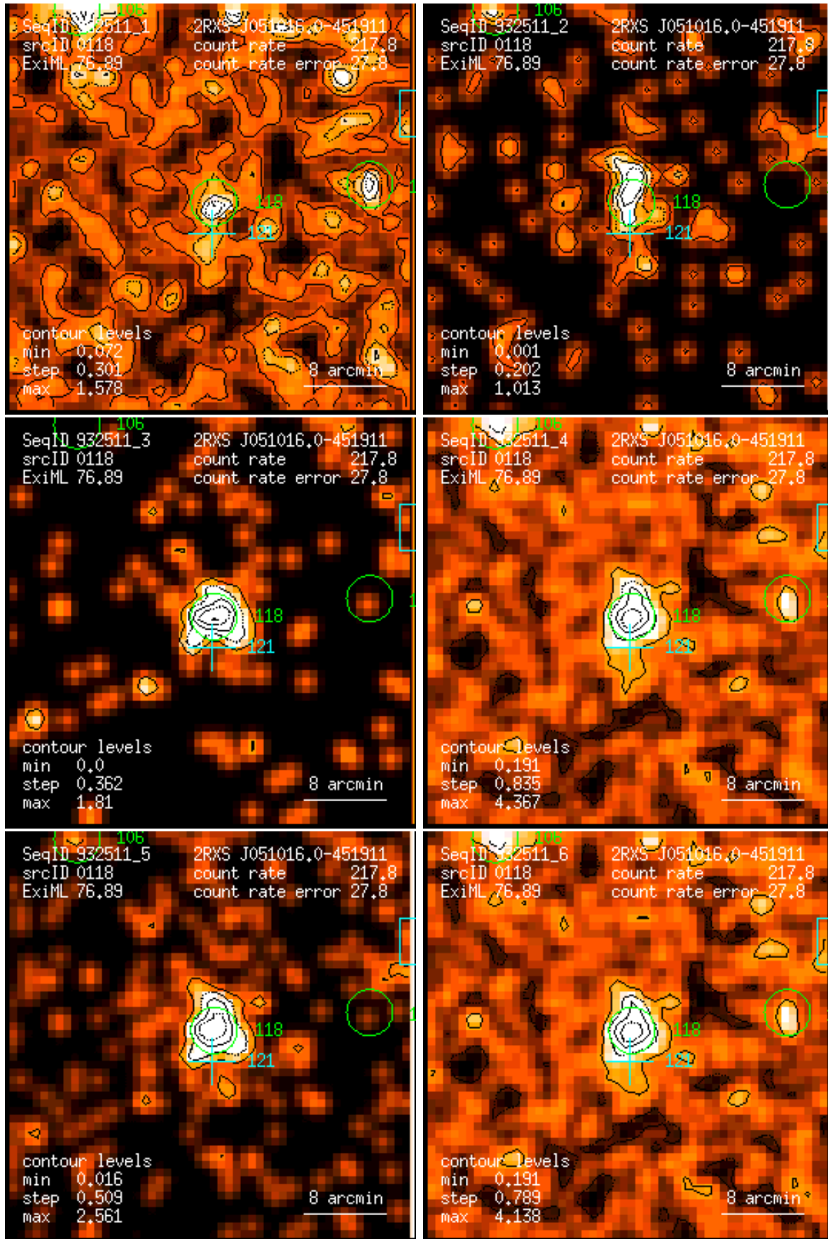
Figure 118: RASS 932511: detection 0118: band rate images, Gaussian filter: (1) PSPC channels 11 – 41, (2) 52 – 90, (3) 91 – 201, (4) 11 – 235, (5) 52 – 201, (6) 11 – 201. Broad band rates in counts/ks. Band rate contour levels in counts/ks/arcmin 2 .
