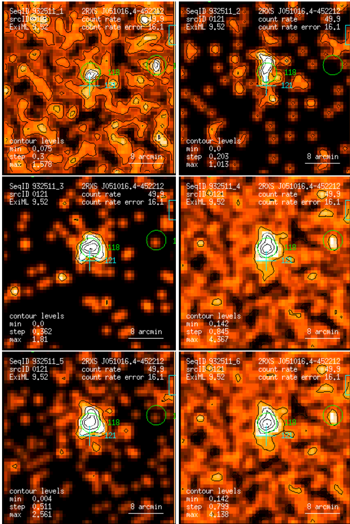
Figure 121: RASS 932511: detection 0121: band rate images, Gaussian filter: (1) PSPC channels 11 – 41, (2) 52 – 90, (3) 91 – 201, (4) 11 – 235, (5) 52 – 201, (6) 11 – 201. Broad band rates in counts/ks. Band rate contour levels in counts/ks/arcmin 2 .
