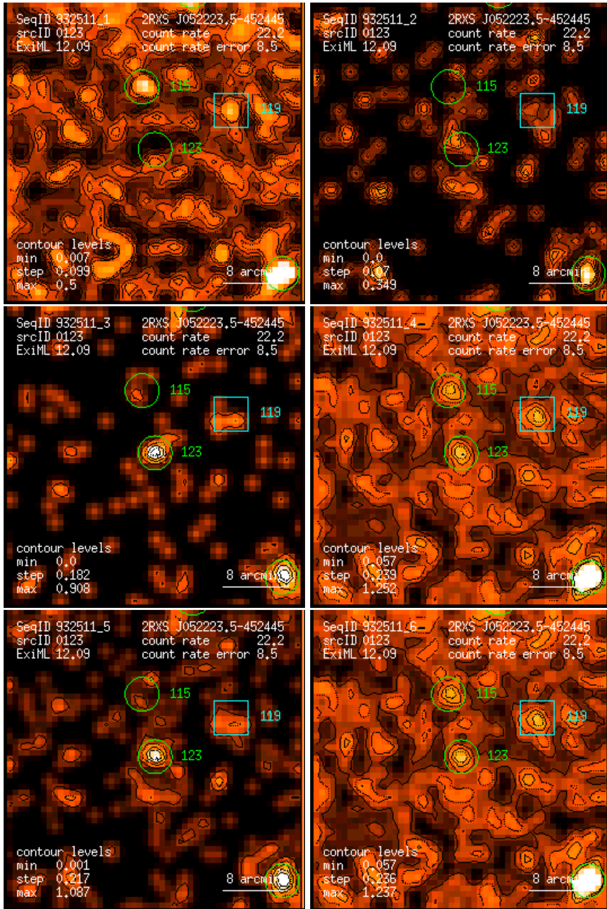
Figure 123: RASS 932511: detection 0123: band rate images, Gaussian filter: (1) PSPC channels 11 – 41, (2) 52 – 90, (3) 91 – 201, (4) 11 – 235, (5) 52 – 201, (6) 11 – 201. Broad band rates in counts/ks. Band rate contour levels in counts/ks/arcmin 2 .
