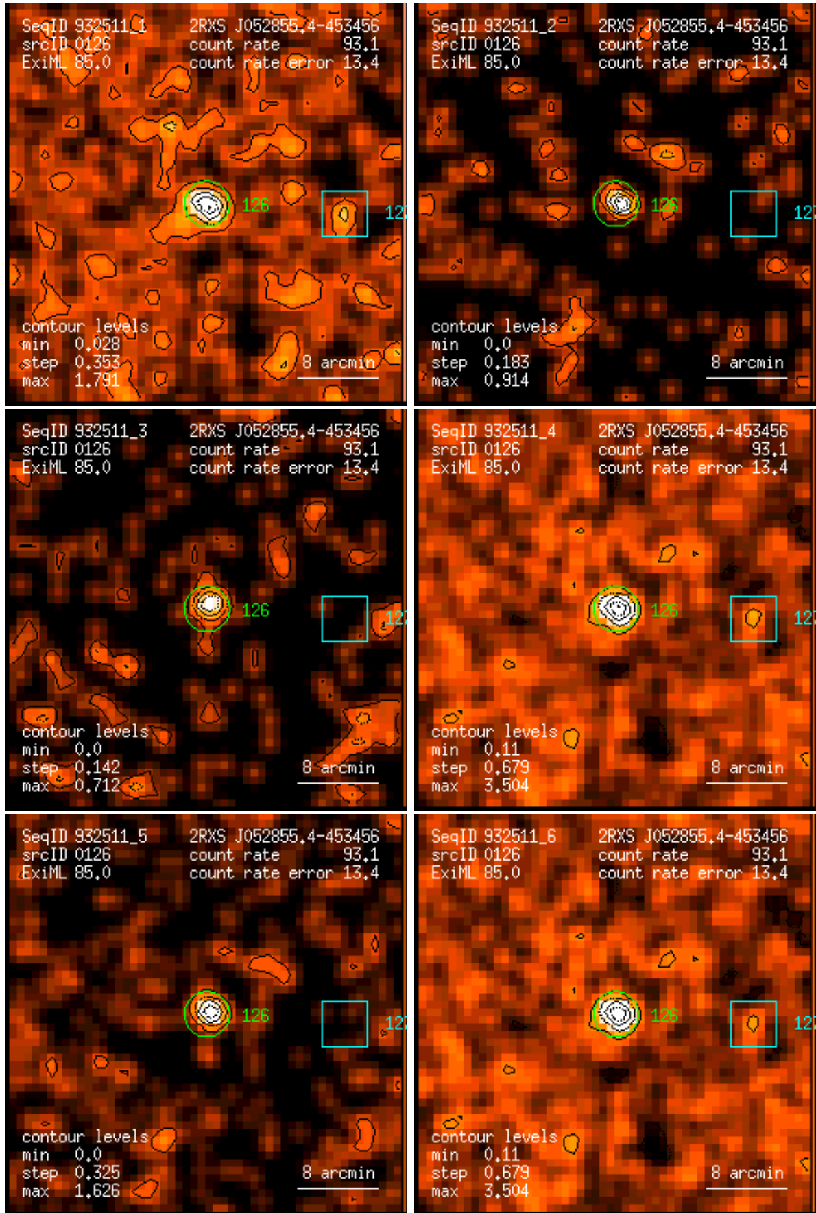
Figure 126: RASS 932511: detection 0126: band rate images, Gaussian filter: (1) PSPC channels 11 – 41, (2) 52 – 90, (3) 91 – 201, (4) 11 – 235, (5) 52 – 201, (6) 11 – 201. Broad band rates in counts/ks. Band rate contour levels in counts/ks/arcmin 2 .
