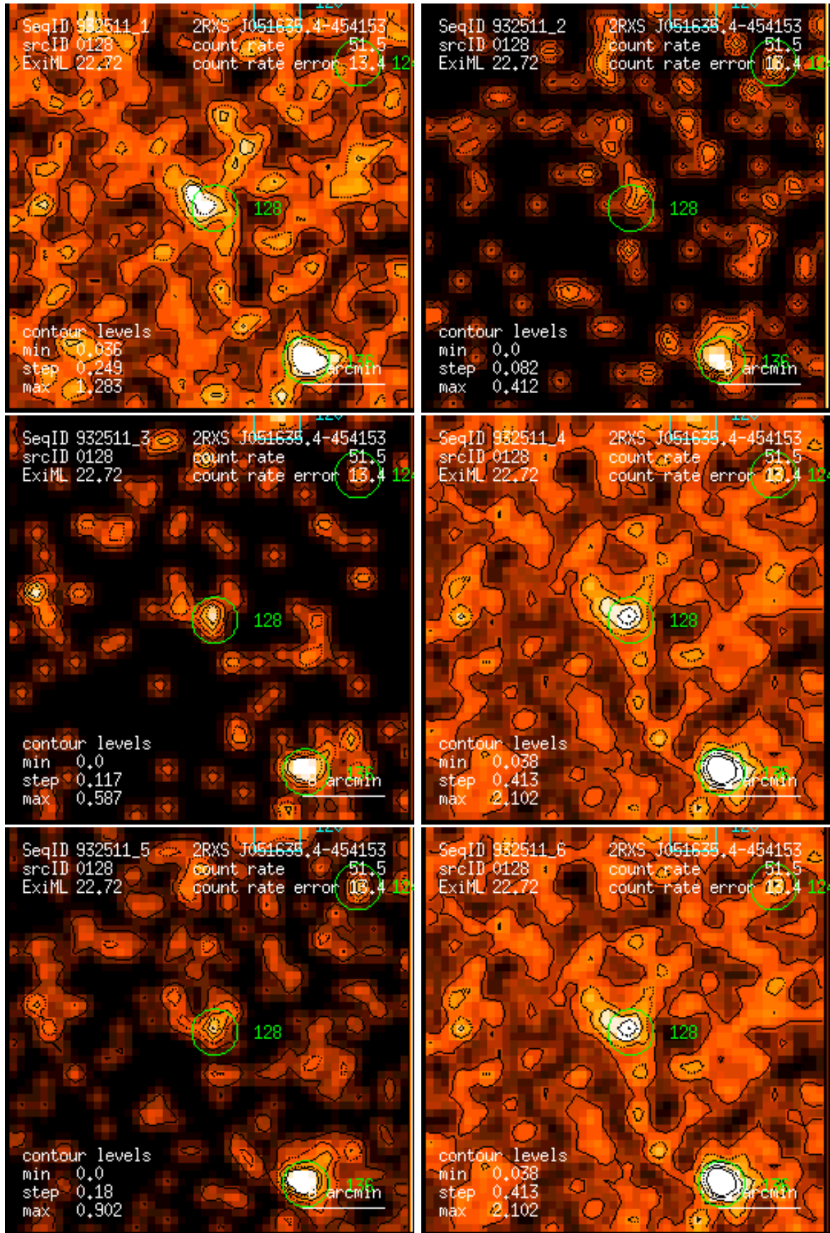
Figure 128: RASS 932511: detection 0128: band rate images, Gaussian filter: (1) PSPC channels 11 – 41, (2) 52 – 90, (3) 91 – 201, (4) 11 – 235, (5) 52 – 201, (6) 11 – 201. Broad band rates in counts/ks. Band rate contour levels in counts/ks/arcmin 2 .
