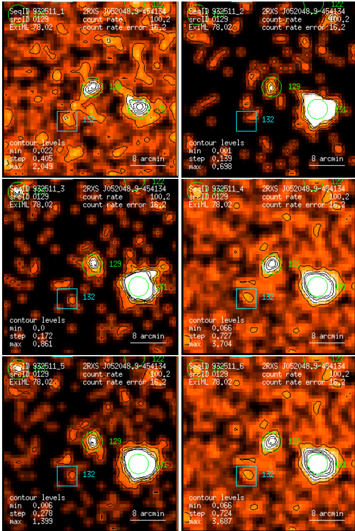
Figure 129: RASS 932511: detection 0129: band rate images, Gaussian filter: (1) PSPC channels 11 – 41, (2) 52 – 90, (3) 91 – 201, (4) 11 – 235, (5) 52 – 201, (6) 11 – 201. Broad band rates in counts/ks. Band rate contour levels in counts/ks/arcmin 2 .
