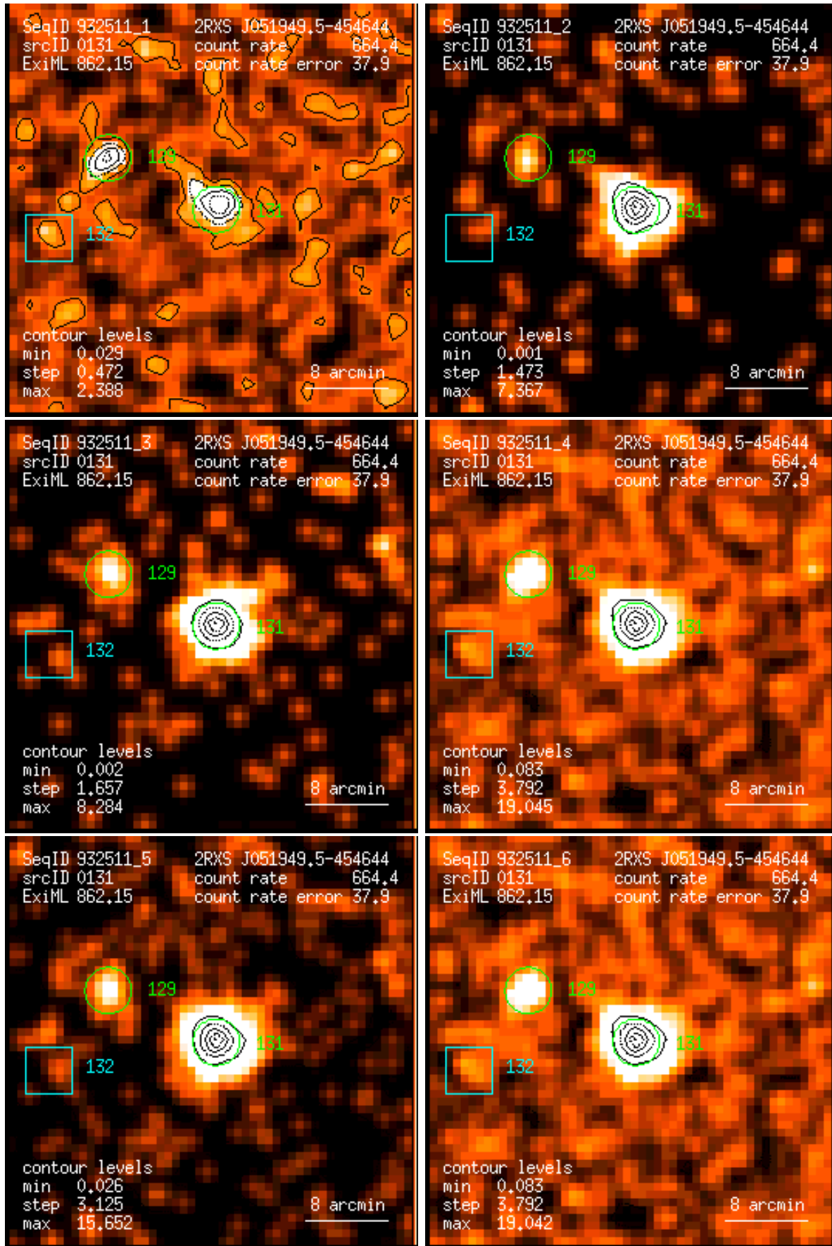
Figure 131: RASS 932511: detection 0131: band rate images, Gaussian filter: (1) PSPC channels 11 – 41, (2) 52 – 90, (3) 91 – 201, (4) 11 – 235, (5) 52 – 201, (6) 11 – 201. Broad band rates in counts/ks. Band rate contour levels in counts/ks/arcmin 2 .
