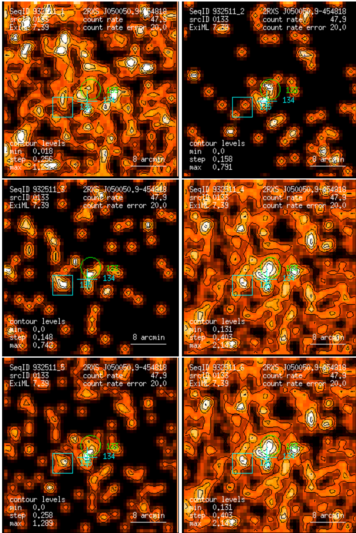
Figure 133: RASS 932511: detection 0133: band rate images, Gaussian filter: (1) PSPC channels 11 – 41, (2) 52 – 90, (3) 91 – 201, (4) 11 – 235, (5) 52 – 201, (6) 11 – 201. Broad band rates in counts/ks. Band rate contour levels in counts/ks/arcmin 2 .
