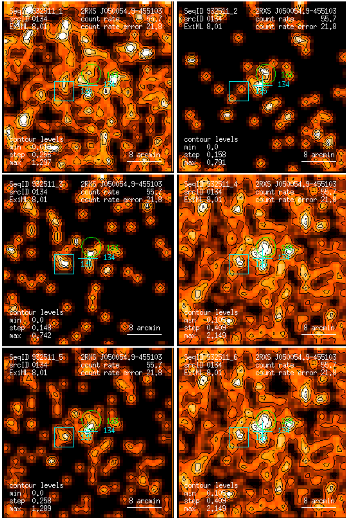
Figure 134: RASS 932511: detection 0134: band rate images, Gaussian filter: (1) PSPC channels 11 – 41, (2) 52 – 90, (3) 91 – 201, (4) 11 – 235, (5) 52 – 201, (6) 11 – 201. Broad band rates in counts/ks. Band rate contour levels in counts/ks/arcmin 2 .
