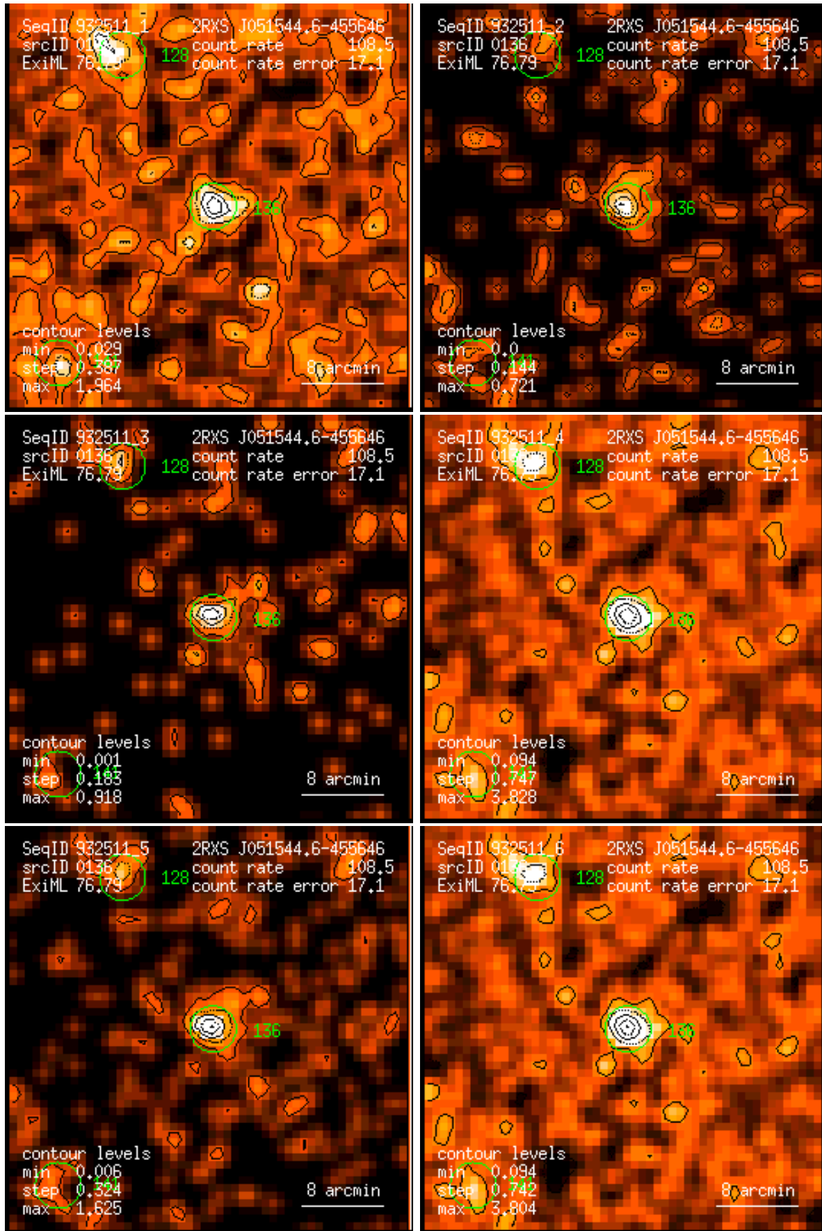
Figure 136: RASS 932511: detection 0136: band rate images, Gaussian filter: (1) PSPPC channels 11 – 41, (2) 52 – 90, (3) 91 – 201, (4) 11 – 235, (5) 52 – 201, (6) 11 – 201. Broad band rates in counts/ks. Band rate contour levels in counts/ks/arcmin 2 .
