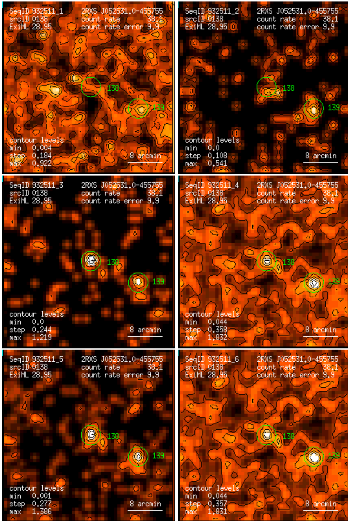
Figure 138: RASS 932511: detection 0138: band rate images, Gaussian filter: (1) PSPC channels 11 – 41, (2) 52 – 90, (3) 91 – 201, (4) 11 – 235, (5) 52 – 201, (6) 11 – 201. Broad band rates in counts/ks. Band rate contour levels in counts/ks/arcmin 2 .
