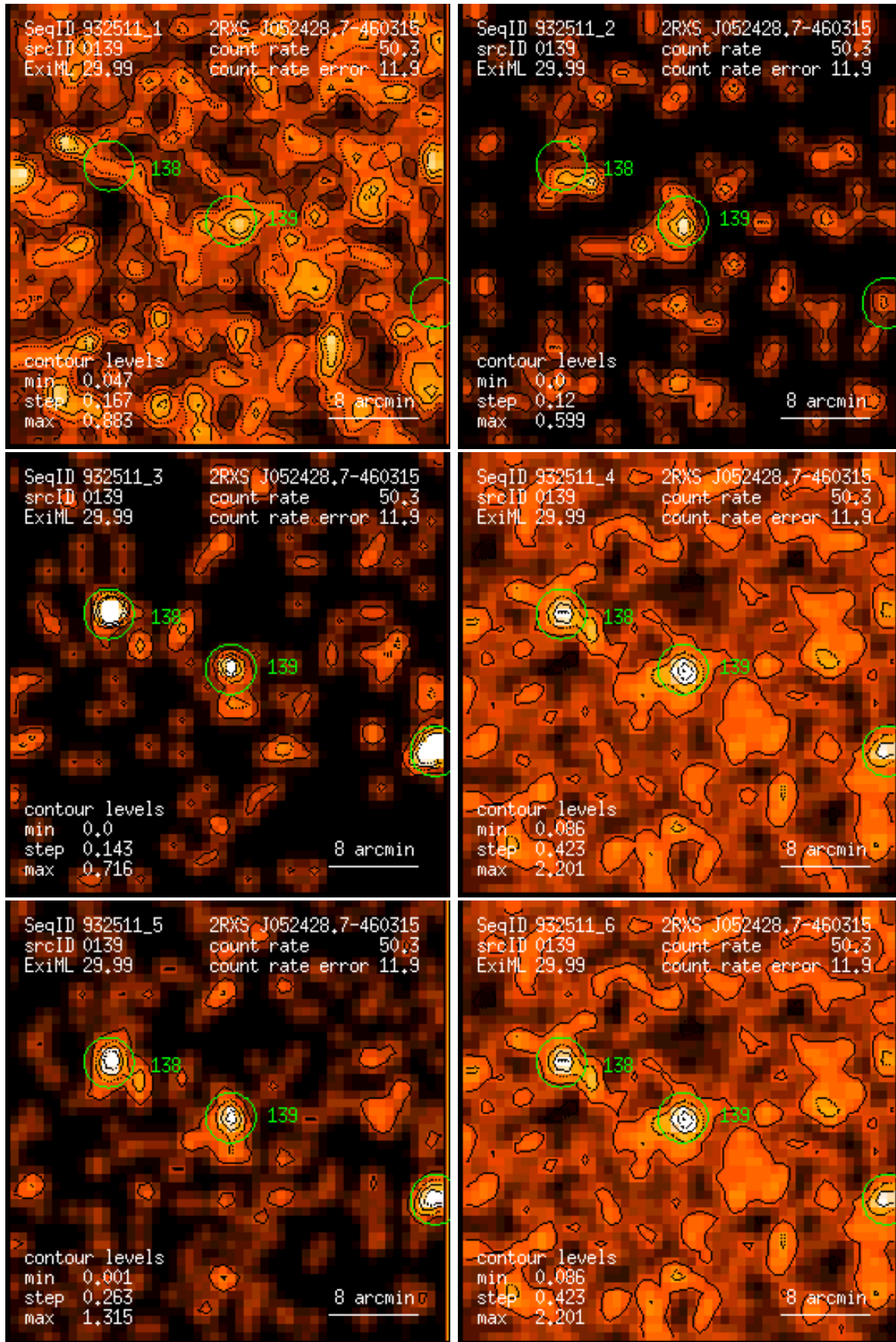
Figure 139: RASS 932511: detection 0139: band rate images, Gaussian filter: (1) PSPC channels 11 – 41, (2) 52 – 90, (3) 91 – 201, (4) 11 – 235, (5) 52 – 201, (6) 11 – 201. Broad band rates in counts/ks. Band rate contour levels in counts/ks/arcmin 2 .
