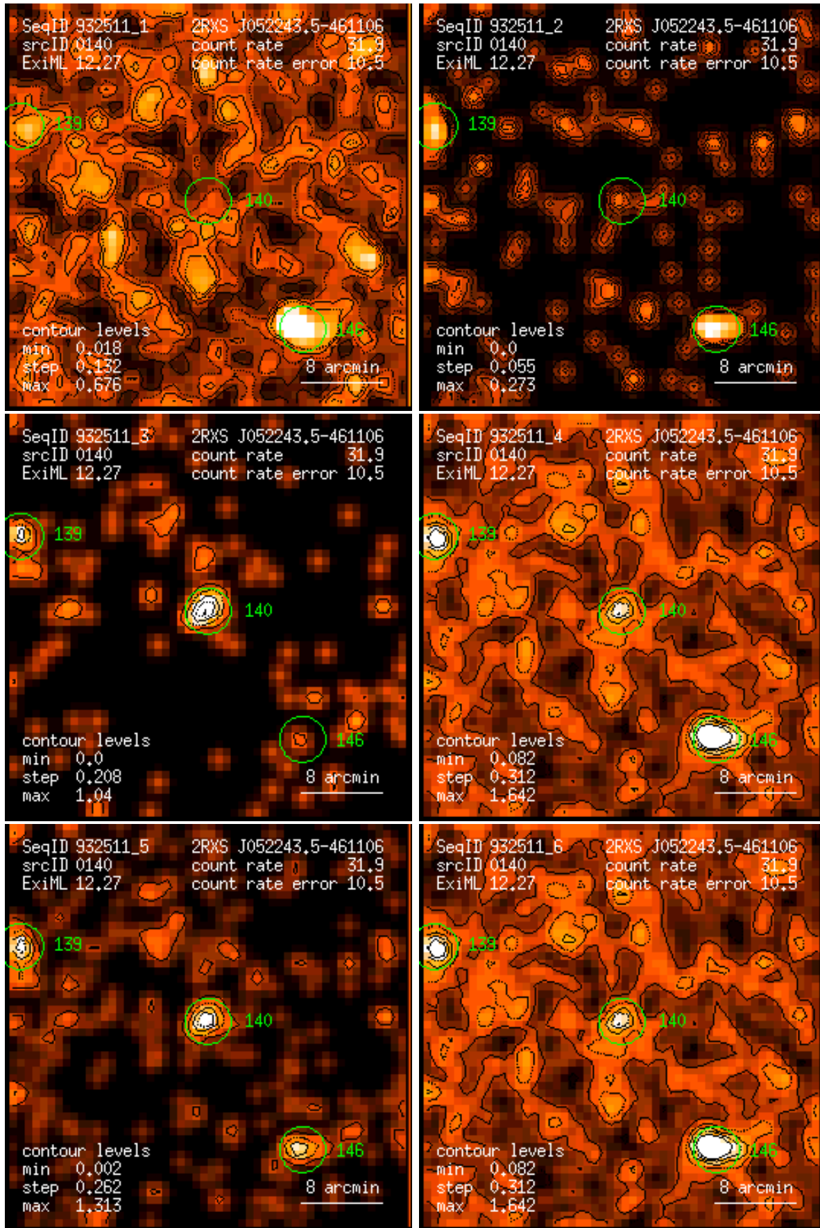
Figure 140: RASS 932511: detection 0140: band rate images, Gaussian filter: (1) PSPC channels 11 – 41, (2) 52 – 90, (3) 91 – 201, (4) 11 – 235, (5) 52 – 201, (6) 11 – 201. Broad band rates in counts/ks. Band rate contour levels in counts/ks/arcmin 2 .
