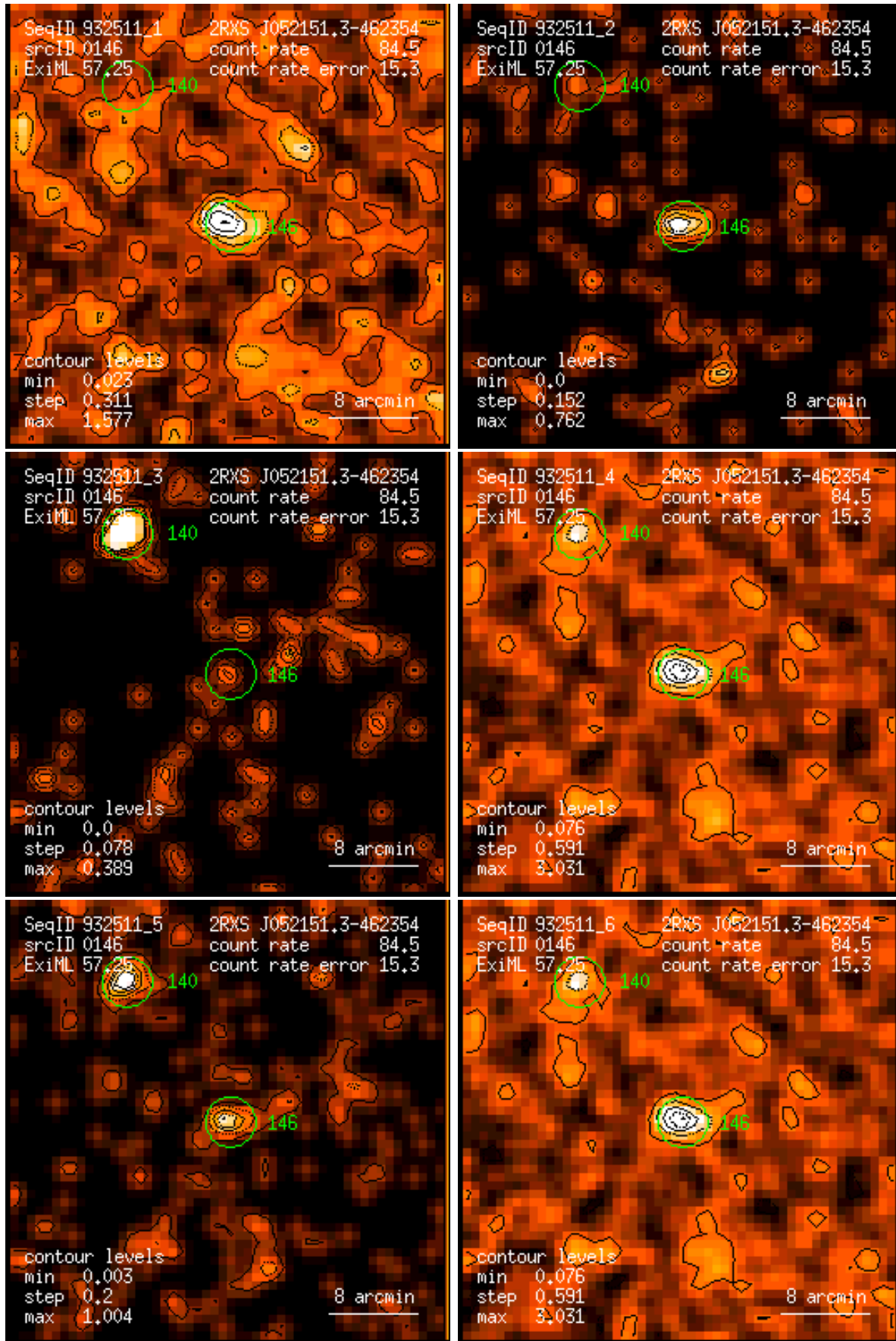
Figure 146: RASS 932511: detection 0146: band rate images, Gaussian filter: (1) PSPC channels 11 – 41, (2) 52 – 90, (3) 91 – 201, (4) 11 – 235, (5) 52 – 201, (6) 11 – 201. Broad band rates in counts/ks. Band rate contour levels in counts/ks/arcmin 2 .
