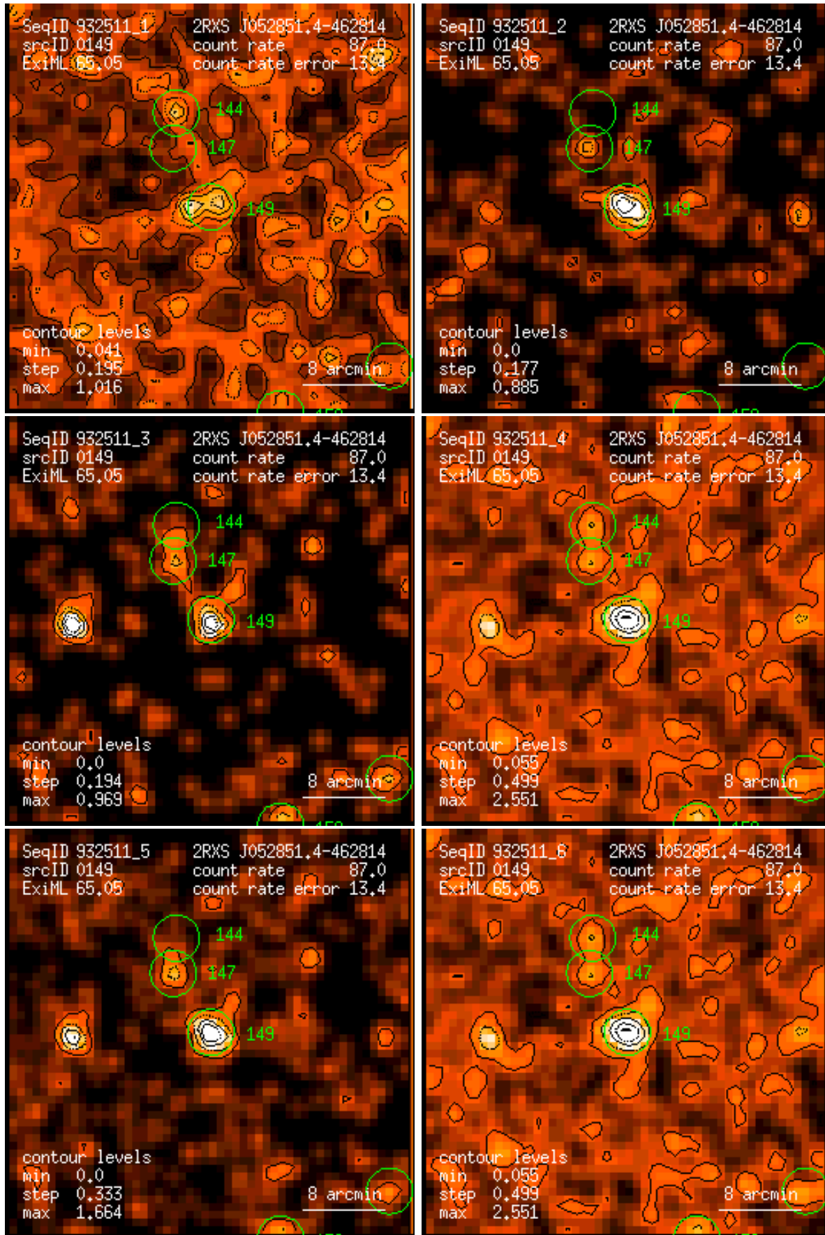
Figure 149: RASS 932511: detection 0149: band rate images, Gaussian filter: (1) PSPC channels 11 – 41, (2) 52 – 90, (3) 91 – 201, (4) 11 – 235, (5) 52 – 201, (6) 11 – 201. Broad band rates in counts/ks. Band rate contour levels in counts/ks/arcmin 2 .
