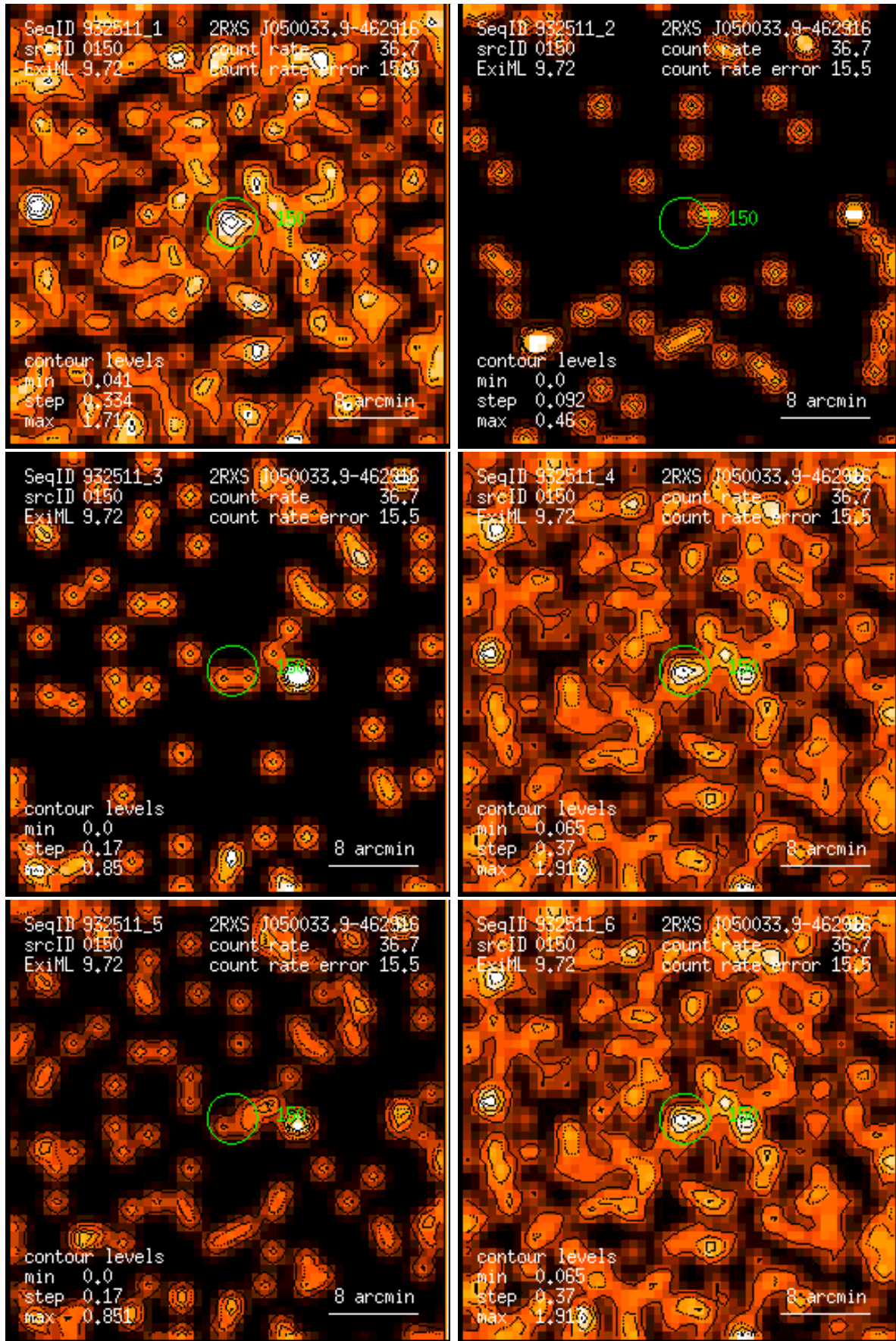
Figure 150: RASS 932511: detection 0150: band rate images, Gaussian filter: (1) PSPC channels 11 – 41, (2) 52 – 90, (3) 91 – 201, (4) 11 – 235, (5) 52 – 201, (6) 11 – 201. Broad band rates in counts/ks. Band rate contour levels in counts/ks/arcmin 2 .
