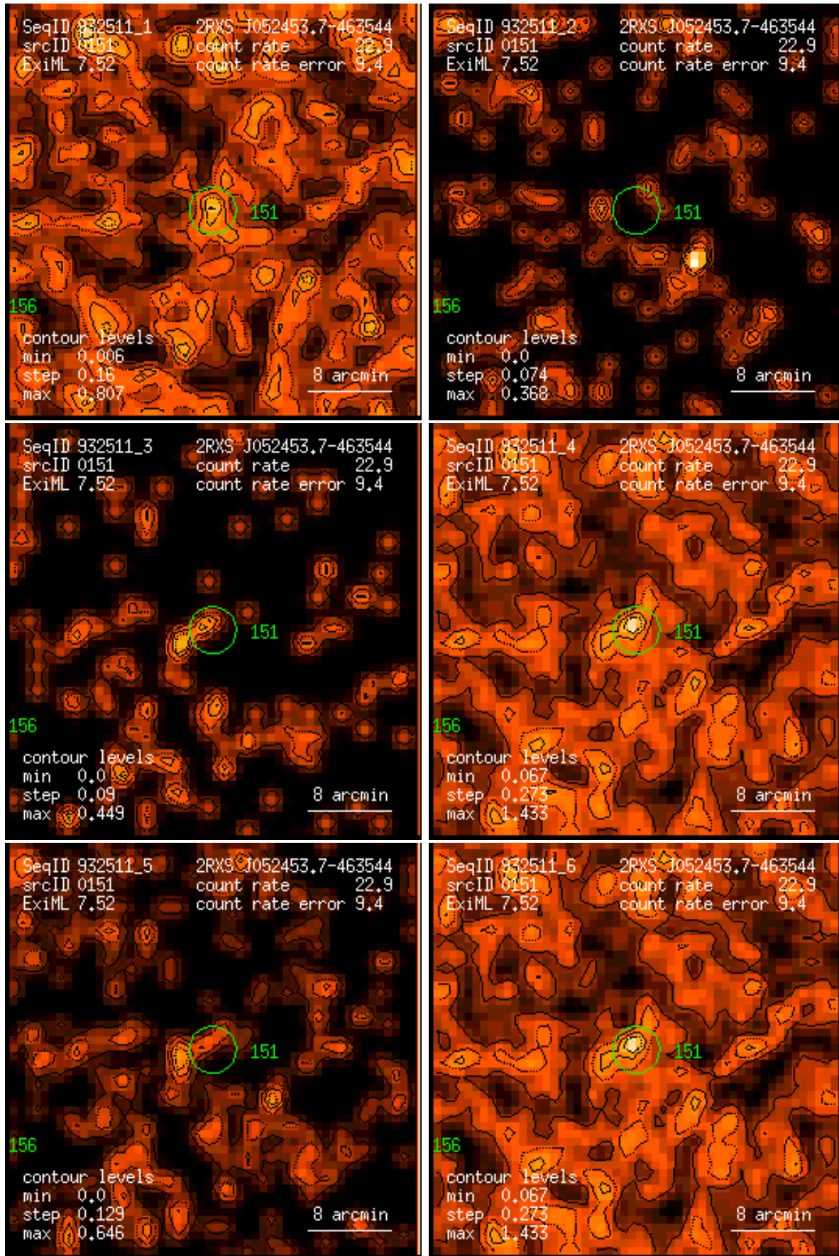
Figure 151: RASS 932511: detection 0151: band rate images, Gaussian filter: (1) PSPC channels 11 – 41, (2) 52 – 90, (3) 91 – 201, (4) 11 – 235, (5) 52 – 201, (6) 11 – 201. Broad band rates in counts/ks. Band rate contour levels in counts/ks/arcmin 2 .
