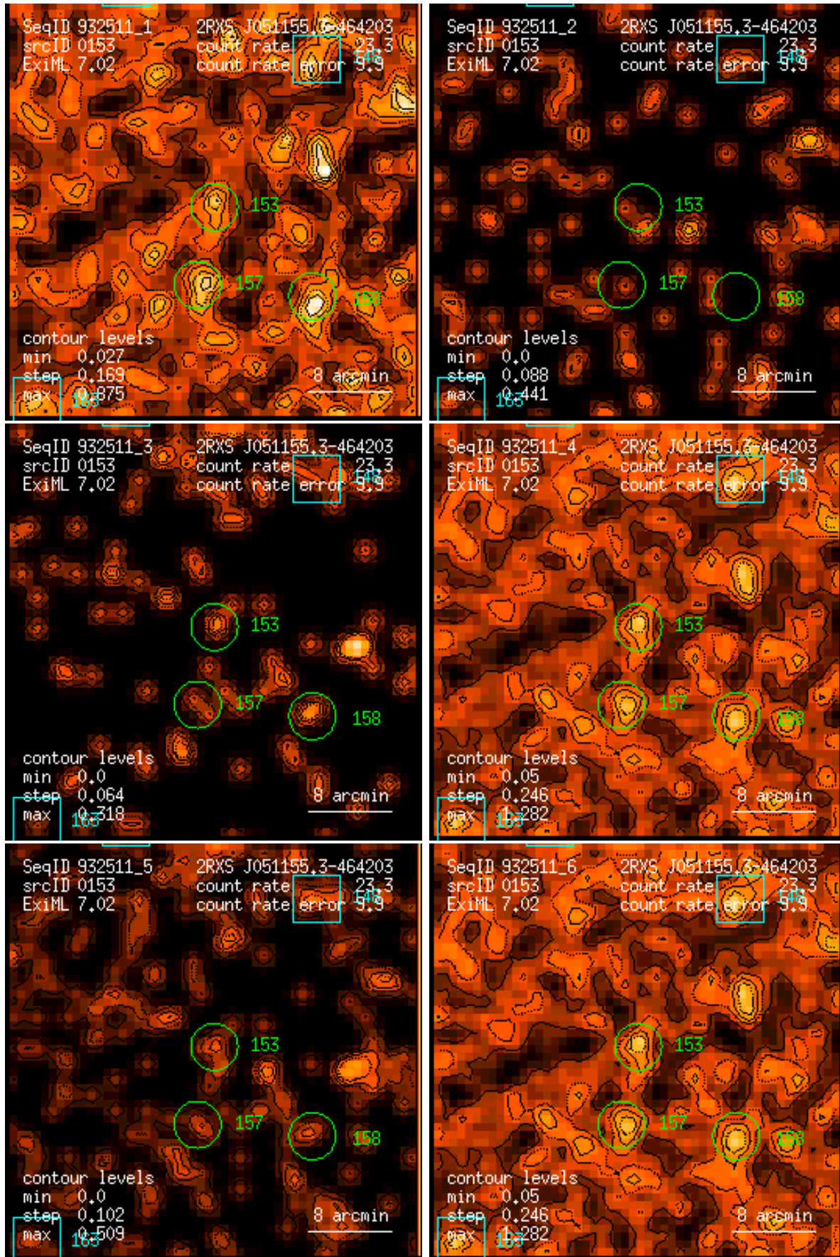
Figure 153: RASS 932511: detection 0153: band rate images, Gaussian filter: (1) PSPC channels 11 – 41, (2) 52 – 90, (3) 91 – 201, (4) 11 – 235, (5) 52 – 201, (6) 11 – 201. Broad band rates in counts/ks. Band rate contour levels in counts/ks/arcmin 2 .
