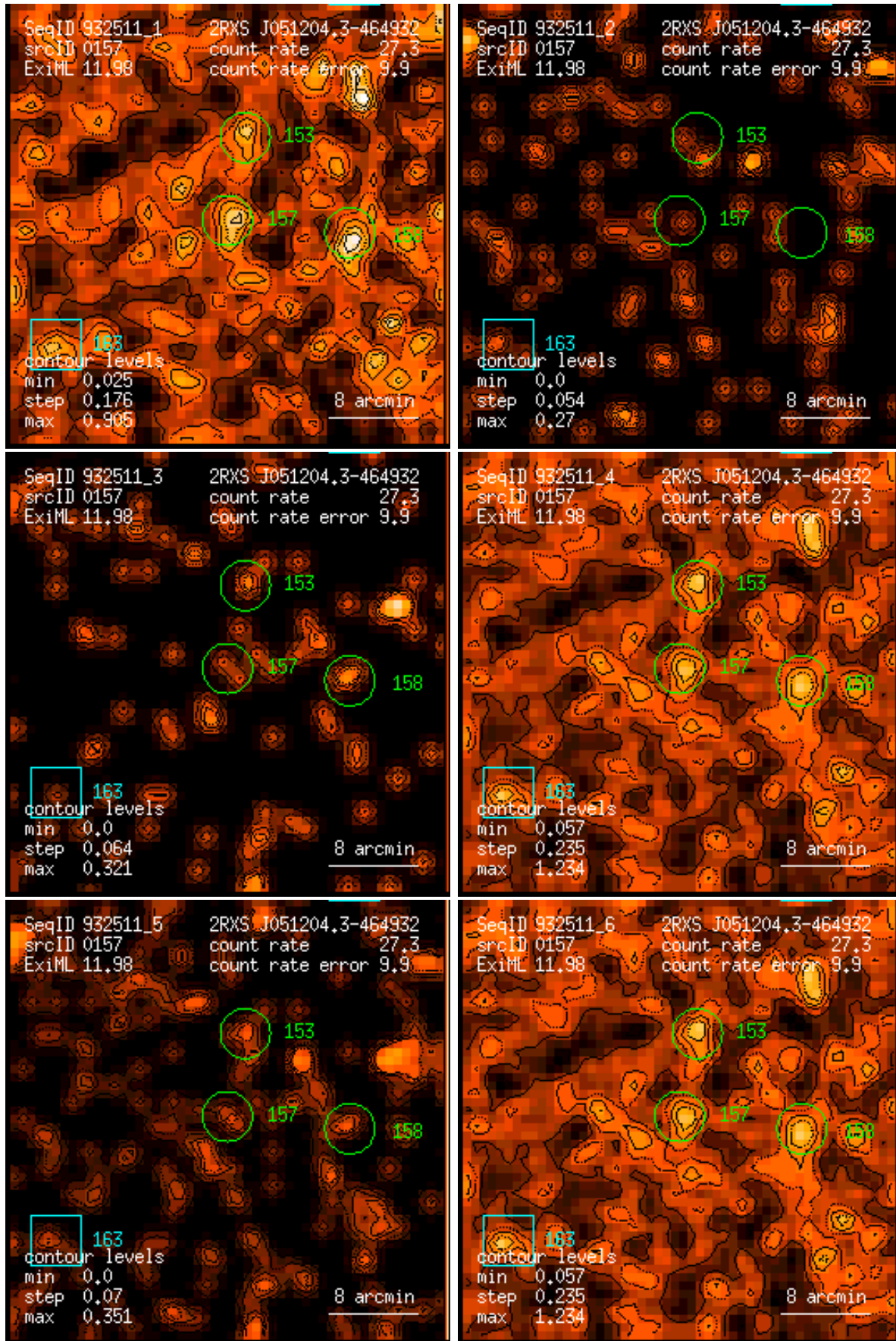
Figure 157: RASS 932511: detection 0157: band rate images, Gaussian filter: (1) PSPC channels 11 – 41, (2) 52 – 90, (3) 91 – 201, (4) 11 – 235, (5) 52 – 201, (6) 11 – 201. Broad band rates in counts/ks. Band rate contour levels in counts/ks/arcmin 2 .
